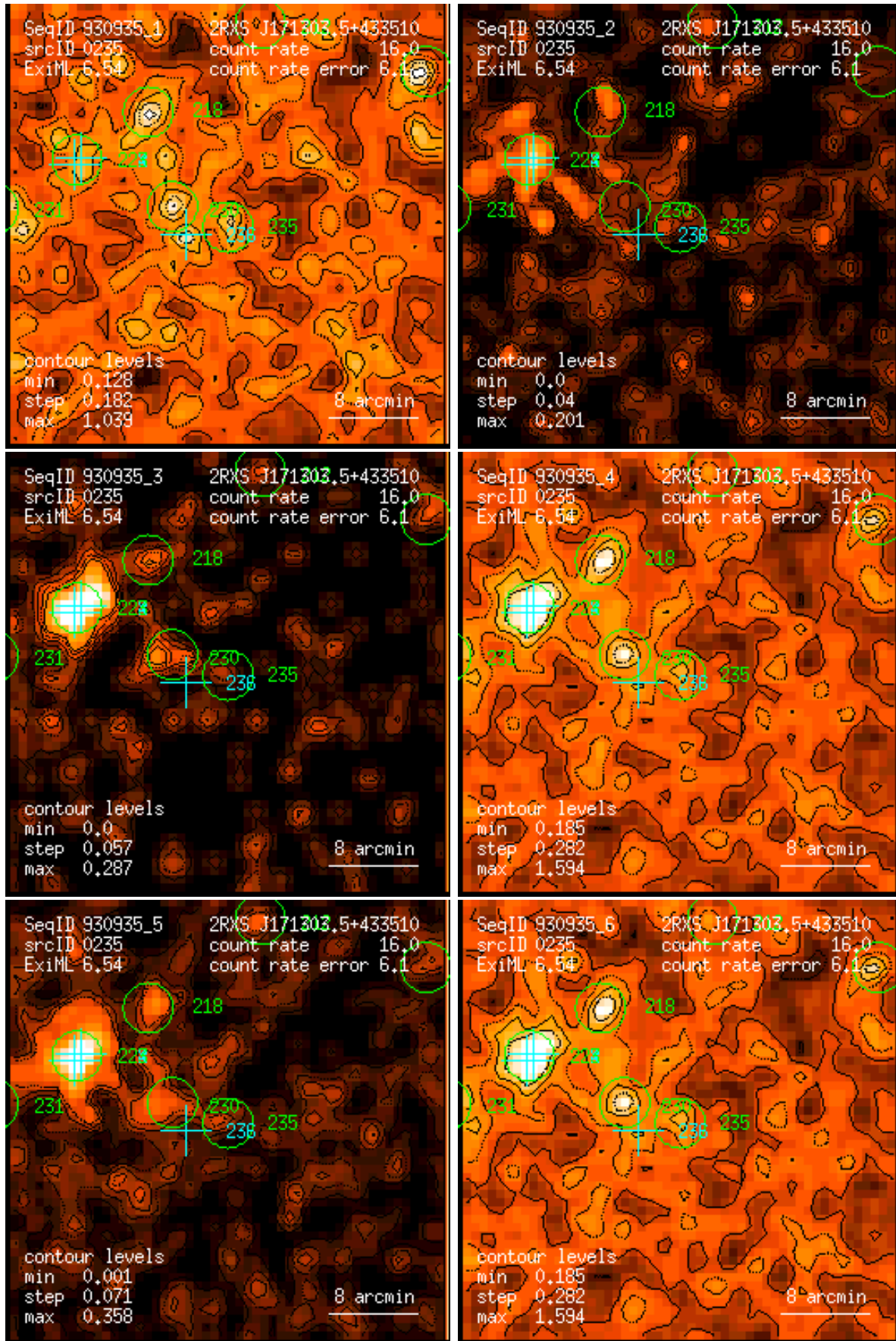
Figure 235: RASS 930935: detection 0235: band rate images, Gaussian filter: (1) PSPC channels 11 – 41, (2) 52 – 90, (3) 91 – 201, (4) 11 – 235, (5) 52 – 201, (6) 11 – 201. Broad band rates in counts/ks. Band rate contour levels in counts/ks/arcmin 2 .
