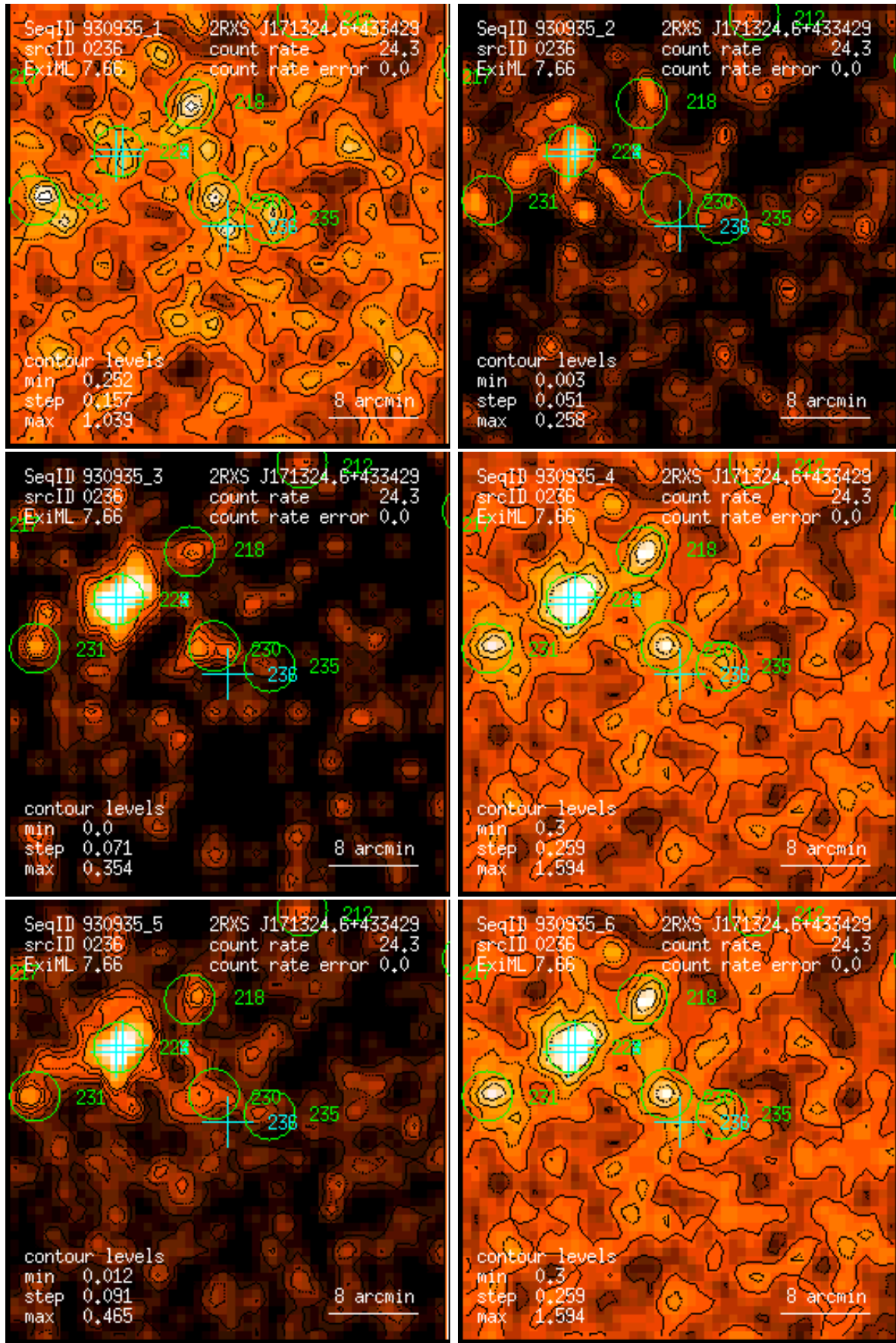
Figure 236: RASS 930935: detection 0236: band rate images, Gaussian filter: (1) PSPC channels 11 – 41, (2) 52 – 90, (3) 91 – 201, (4) 11 – 235, (5) 52 – 201, (6) 11 – 201. Broad band rates in counts/ks. Band rate contour levels in counts/ks/arcmin 2 .
