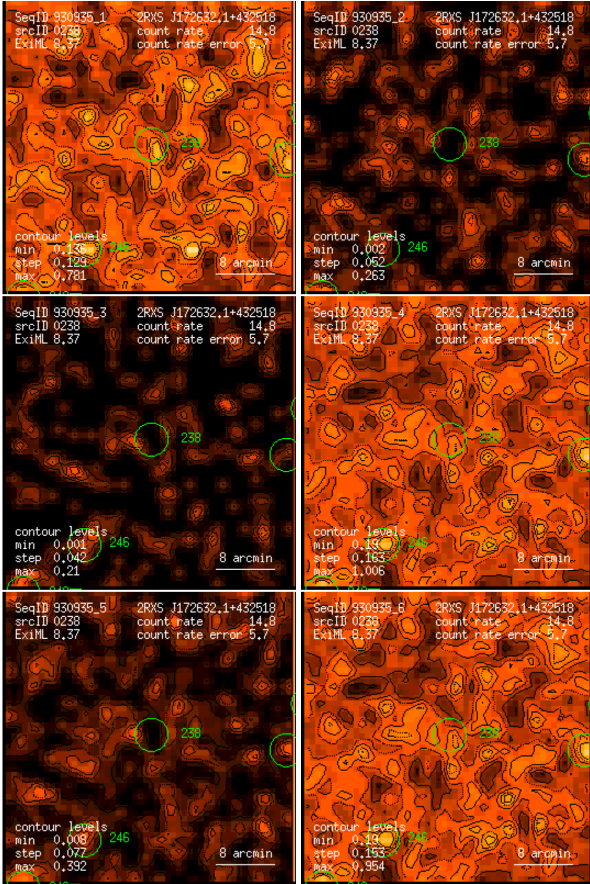
Figure 238: RASS 930935: detection 0238: band rate images, Gaussian filter: (1) PSPC channels 11 – 41, (2) 52 – 90, (3) 91 – 201, (4) 11 – 235, (5) 52 – 201, (6) 11 – 201. Broad band rates in counts/ks. Band rate contour levels in counts/ks/arcmin 2 .
