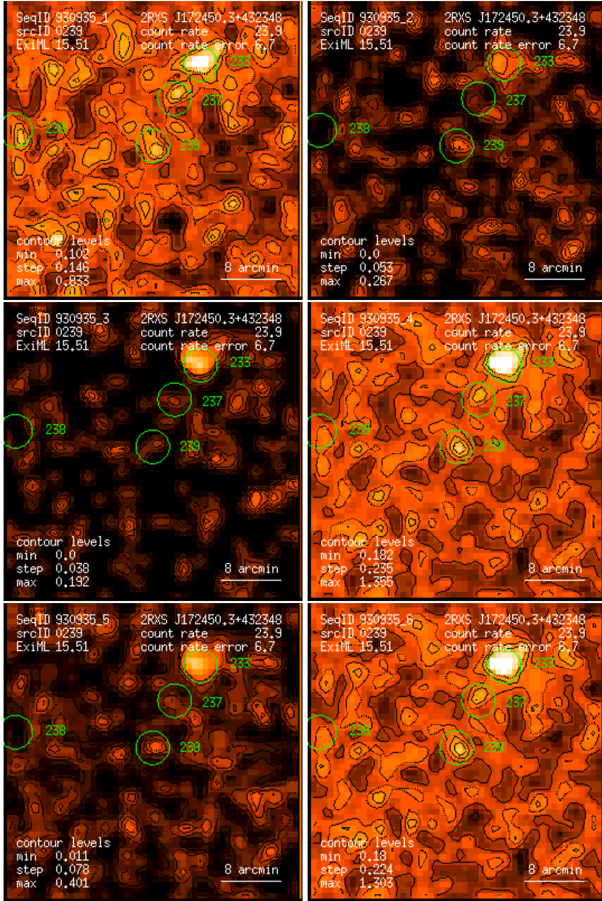
Figure 239: RASS 930935: detection 0239: band rate images, Gaussian filter: (1) PSPC channels 11 – 41, (2) 52 – 90, (3) 91 – 201, (4) 11 – 235, (5) 52 – 201, (6) 11 – 201. Broad band rates in counts/ks. Band rate contour levels in counts/ks/arcmin 2 .
