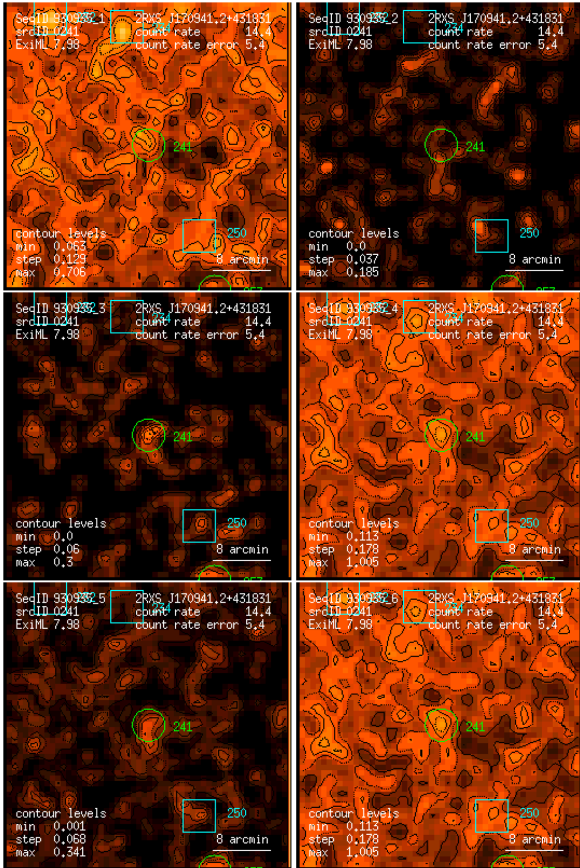
Figure 241: RASS 930935: detection 0241: band rate images, Gaussian filter: (1) PSPC channels 11 – 41, (2) 52 – 90, (3) 91 – 201, (4) 11 – 235, (5) 52 – 201, (6) 11 – 201. Broad band rates in counts/ks. Band rate contour levels in counts/ks/arcmin 2 .
