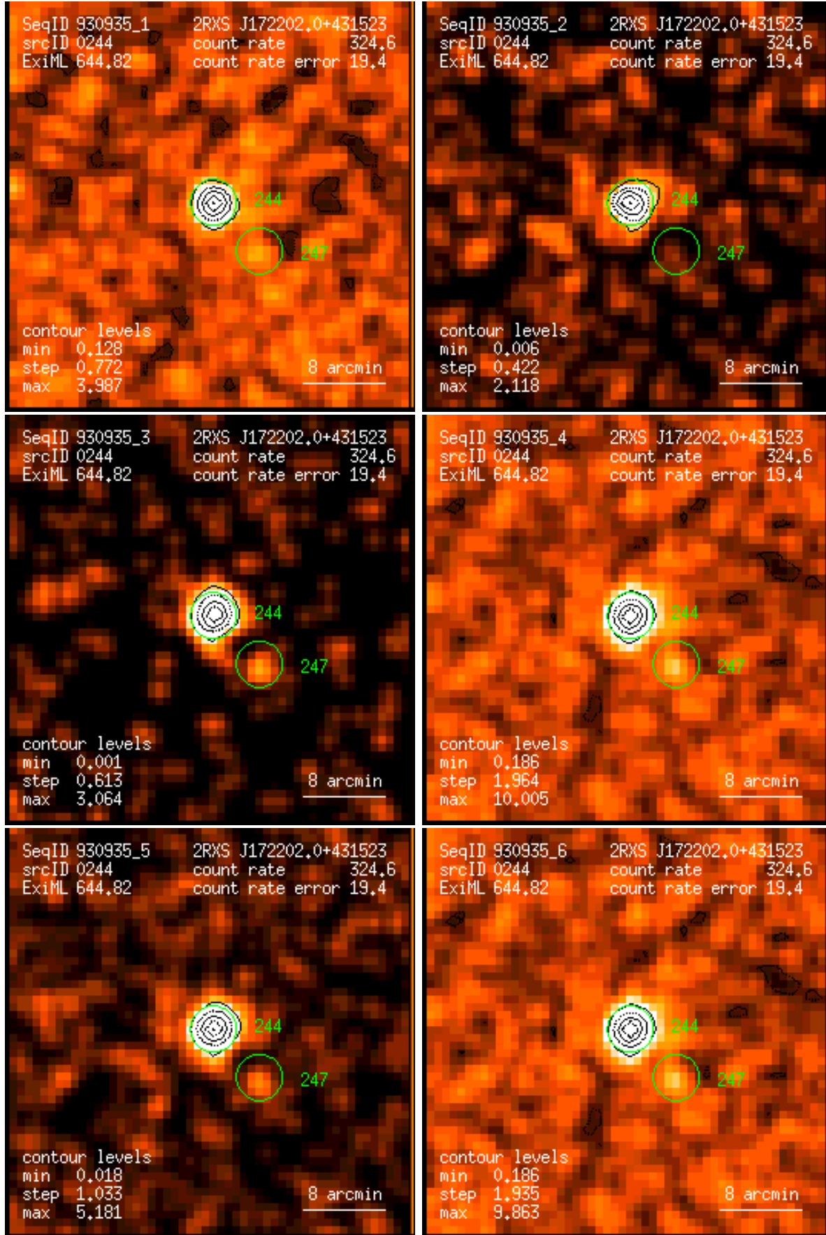
Figure 244: RASS 930935: detection 0244: band rate images, Gaussian filter: (1) PSPC channels 11 – 41, (2) 52 – 90, (3) 91 – 201, (4) 11 – 235, (5) 52 – 201, (6) 11 – 201. Broad band rates in counts/ks. Band rate contour levels in counts/ks/arcmin 2 .
