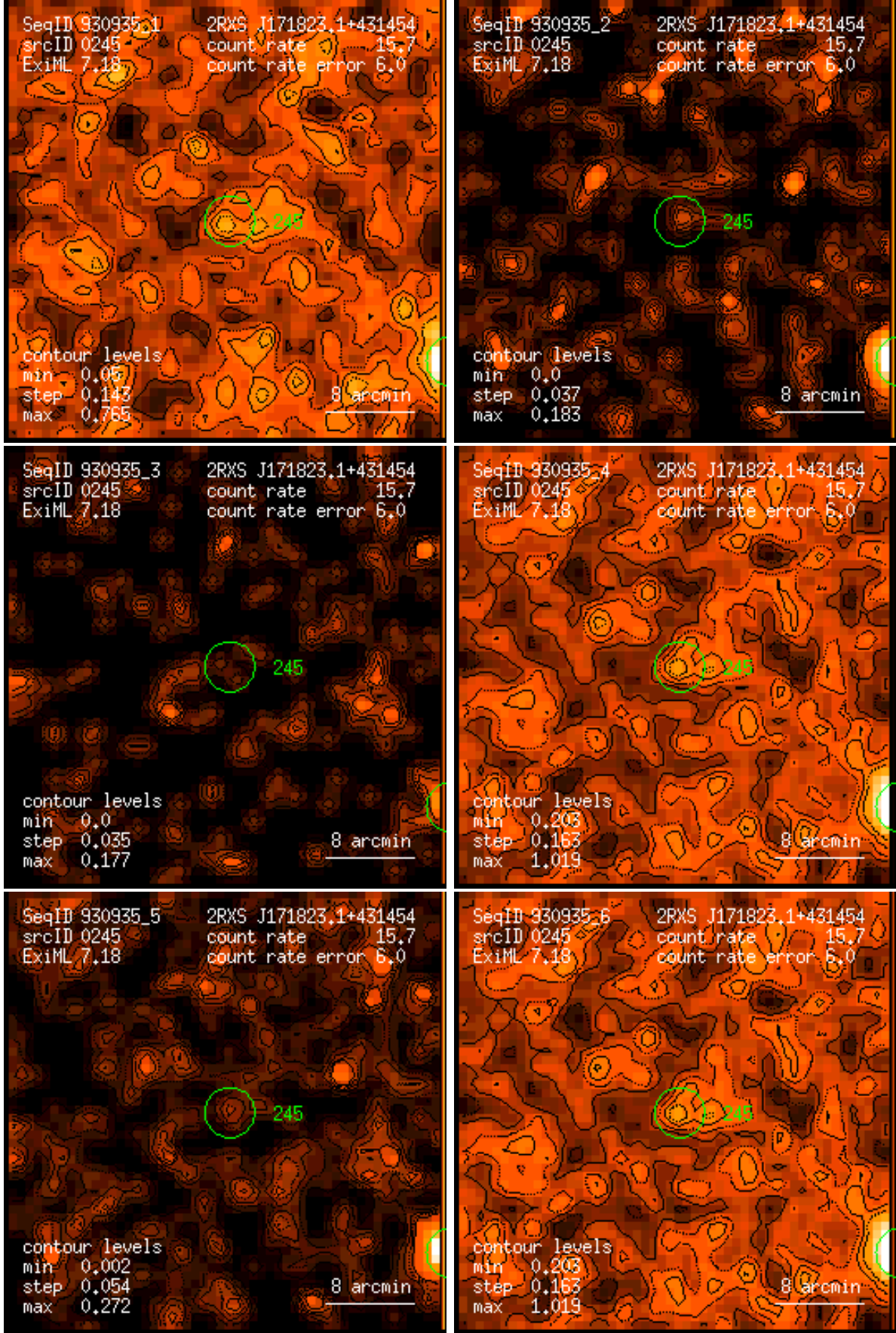
Figure 245: RASS 930935: detection 0245: band rate images, Gaussian filter: (1) PSPC channels 11 – 41, (2) 52 – 90, (3) 91 – 201, (4) 11 – 235, (5) 52 – 201, (6) 11 – 201. Broad band rates in counts/ks. Band rate contour levels in counts/ks/arcmin 2 .
