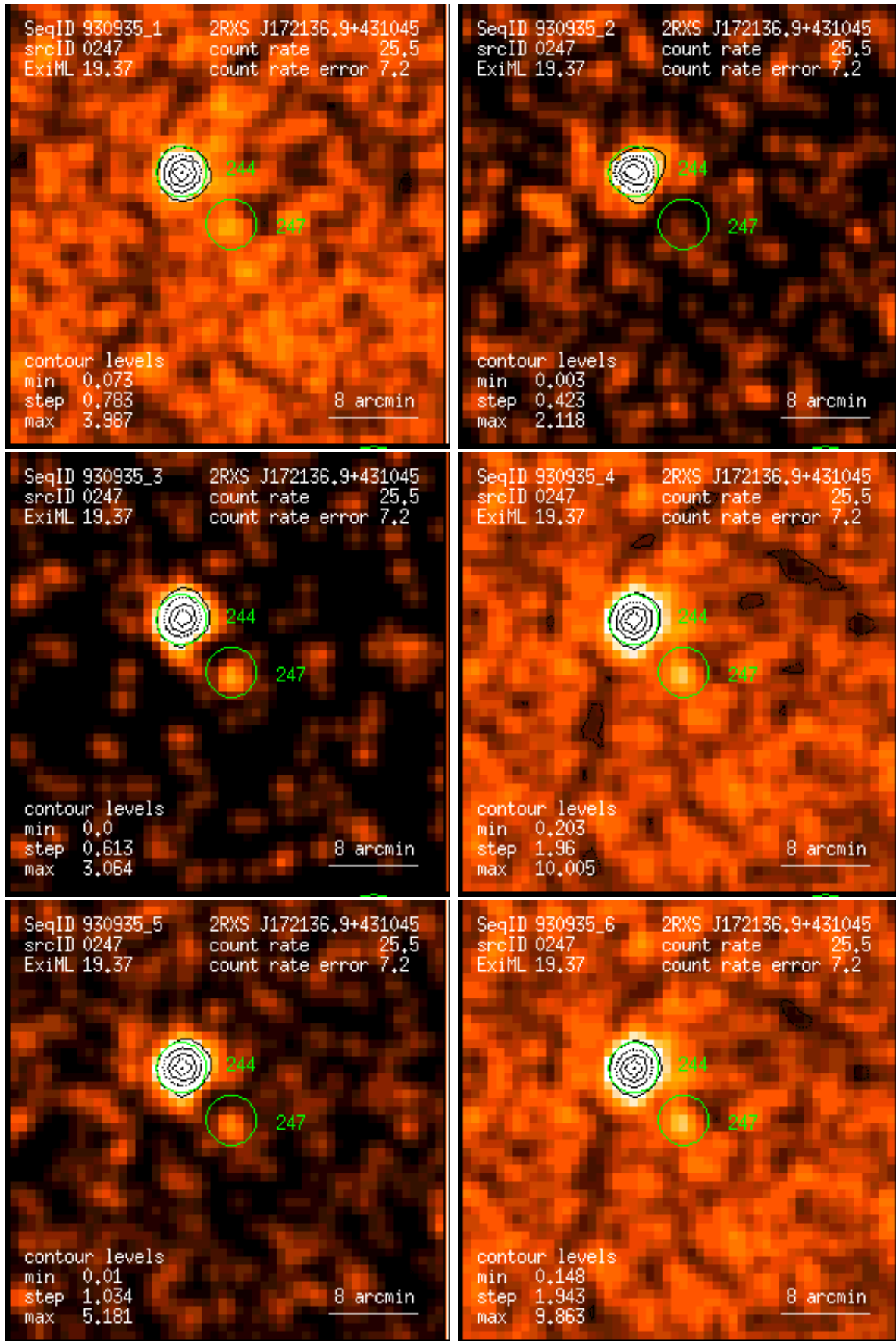
Figure 247: RASS 930935: detection 0247: band rate images, Gaussian filter: (1) PSPC channels 11 – 41, (2) 52 – 90, (3) 91 – 201, (4) 11 – 235, (5) 52 – 201, (6) 11 – 201. Broad band rates in counts/ks. Band rate contour levels in counts/ks/arcmin 2 .
