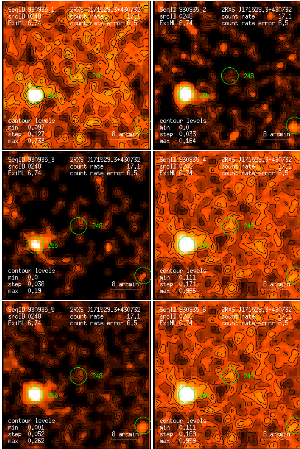
Figure 248: RASS 930935: detection 0248: band rate images, Gaussian filter: (1) PSPC channels 11 – 41, (2) 52 – 90, (3) 91 – 201, (4) 11 – 235, (5) 52 – 201, (6) 11 – 201. Broad band rates in counts/ks. Band rate contour levels in counts/ks/arcmin 2 .
