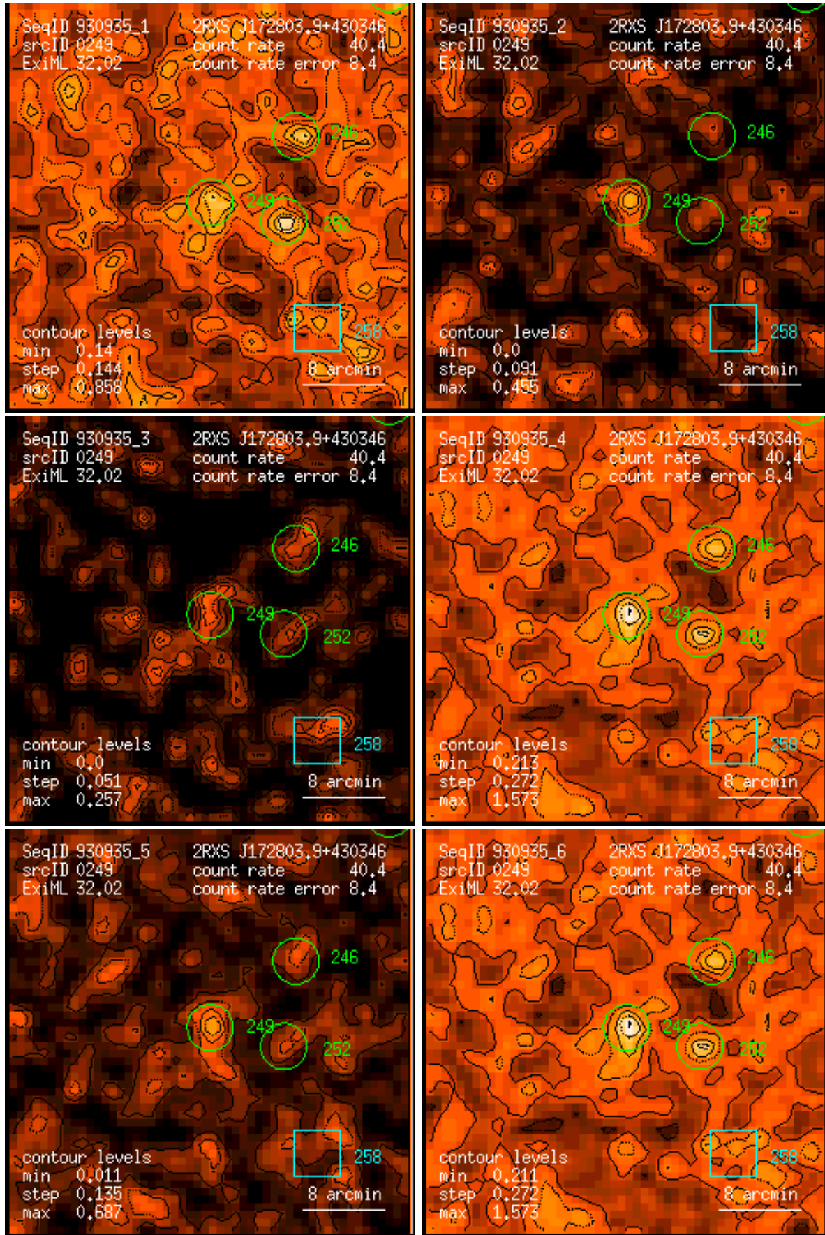
Figure 249: RASS 930935: detection 0249: band rate images, Gaussian filter: (1) PSPC channels 11 – 41, (2) 52 – 90, (3) 91 – 201, (4) 11 – 235, (5) 52 – 201, (6) 11 – 201. Broad band rates in counts/ks. Band rate contour levels in counts/ks/arcmin 2 .
