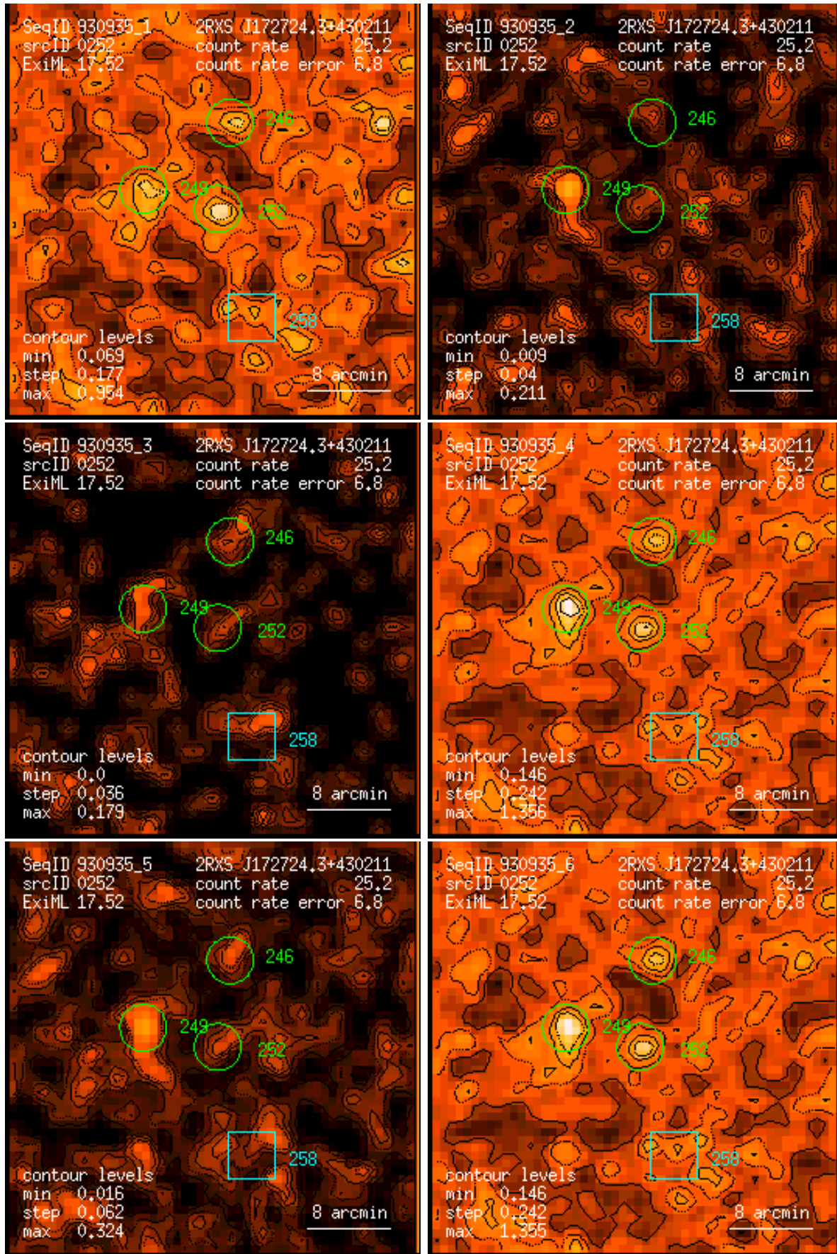
Figure 252: RASS 930935: detection 0252: band rate images, Gaussian filter: (1) PSPC channels 11 – 41, (2) 52 – 90, (3) 91 – 201, (4) 11 – 235, (5) 52 – 201, (6) 11 – 201. Broad band rates in counts/ks. Band rate contour levels in counts/ks/arcmin 2 .
