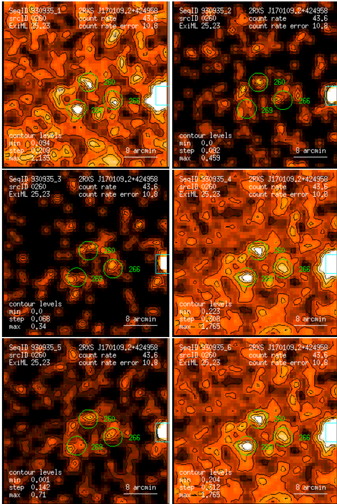
Figure 260: RASS 930935: detection 0260: band rate images, Gaussian filter: (1) PSPC channels 11 – 41, (2) 52 – 90, (3) 91 – 201, (4) 11 – 235, (5) 52 – 201, (6) 11 – 201. Broad band rates in counts/ks. Band rate contour levels in counts/ks/arcmin 2 .
