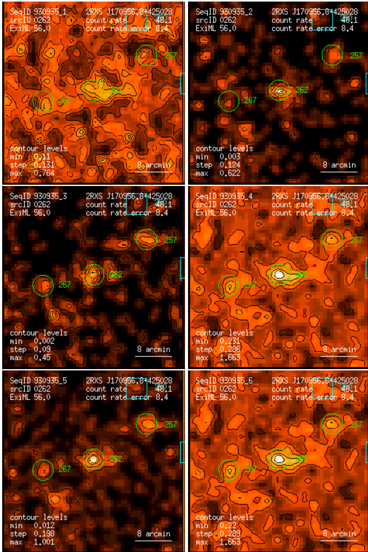
Figure 262: RASS 930935: detection 0262: band rate images, Gaussian filter: (1) PSPC channels 11 – 41, (2) 52 – 90, (3) 91 – 201, (4) 11 – 235, (5) 52 – 201, (6) 11 – 201. Broad band rates in counts/ks. Band rate contour levels in counts/ks/arcmin 2 .
