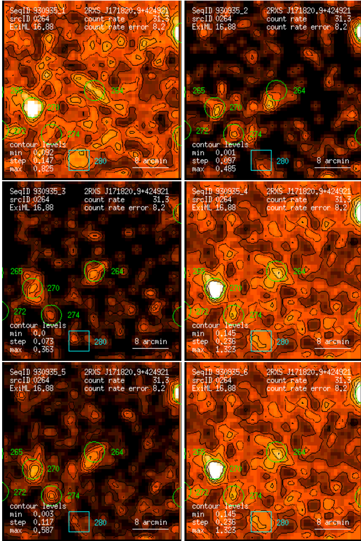
Figure 264: RASS 930935: detection 0264: band rate images, Gaussian filter: (1) PSPC channels 11 – 41, (2) 52 – 90, (3) 91 – 201, (4) 11 – 235, (5) 52 – 201, (6) 11 – 201. Broad band rates in counts/ks. Band rate contour levels in counts/ks/arcmin 2 .
