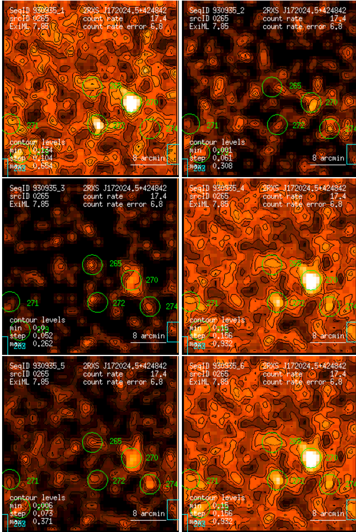
Figure 265: RASS 930935: detection 0265: band rate images, Gaussian filter: (1) PSPC channels 11 – 41, (2) 52 – 90, (3) 91 – 201, (4) 11 – 235, (5) 52 – 201, (6) 11 – 201. Broad band rates in counts/ks. Band rate contour levels in counts/ks/arcmin 2 .
