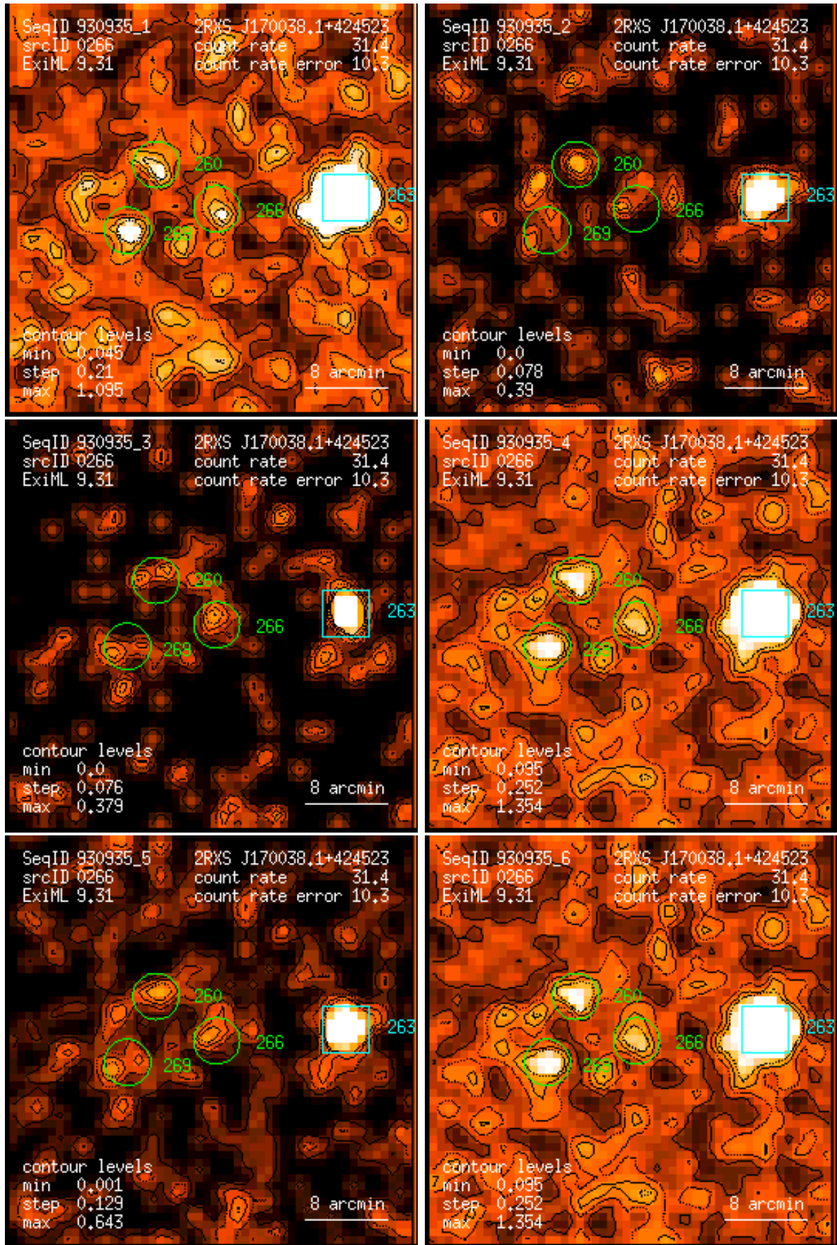
Figure 266: RASS 930935: detection 0266: band rate images, Gaussian filter: (1) PSPC channels 11 – 41, (2) 52 – 90, (3) 91 – 201, (4) 11 – 235, (5) 52 – 201, (6) 11 – 201. Broad band rates in counts/ks. Band rate contour levels in counts/ks/arcmin 2 .
