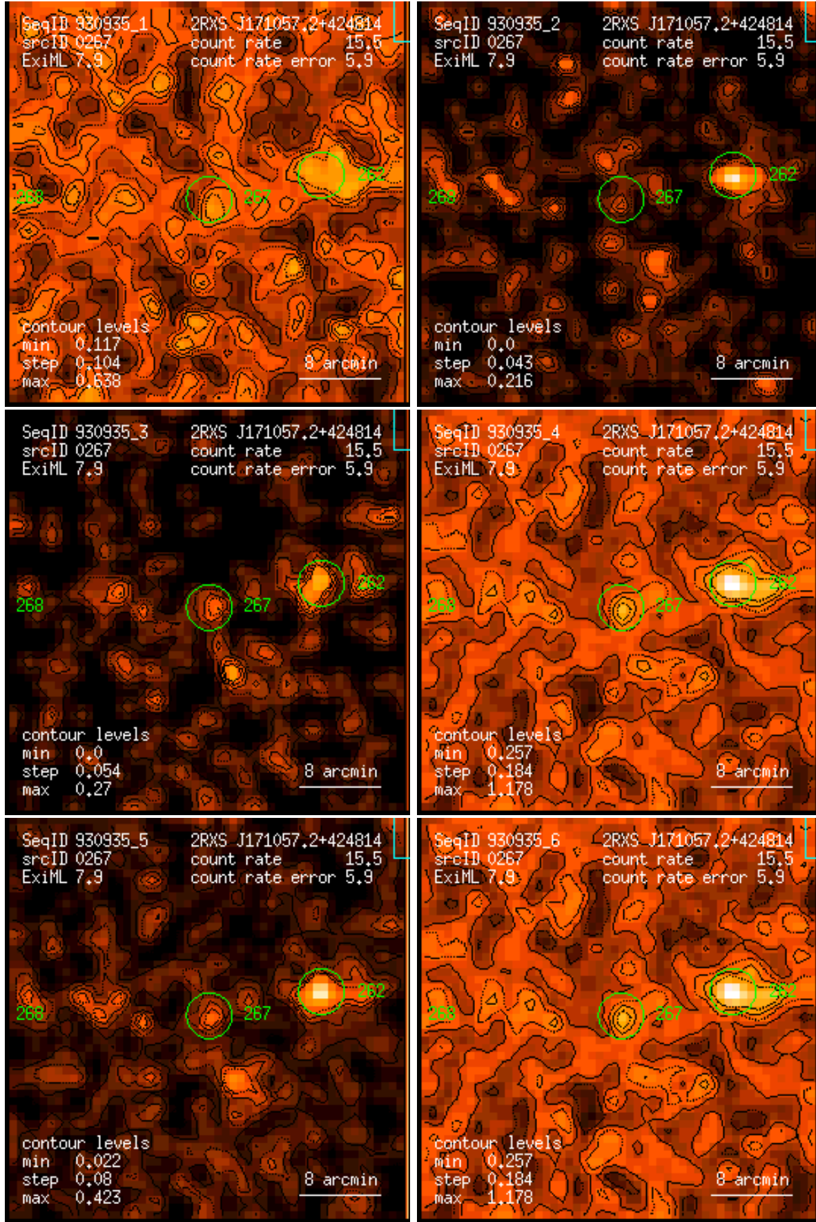
Figure 267: RASS 930935: detection 0267: band rate images, Gaussian filter: (1) PSPC channels 11 – 41, (2) 52 – 90, (3) 91 – 201, (4) 11 – 235, (5) 52 – 201, (6) 11 – 201. Broad band rates in counts/ks. Band rate contour levels in counts/ks/arcmin 2 .
