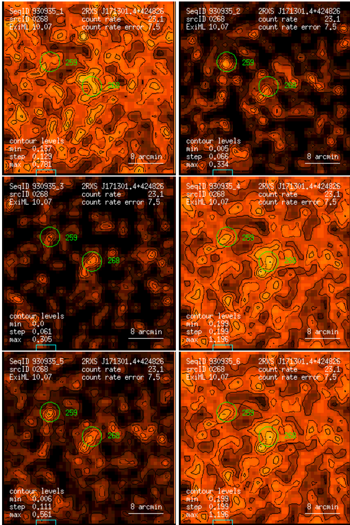
Figure 268: RASS 930935: detection 0268: band rate images, Gaussian filter: (1) PSPC channels 11 – 41, (2) 52 – 90, (3) 91 – 201, (4) 11 – 235, (5) 52 – 201, (6) 11 – 201. Broad band rates in counts/ks. Band rate contour levels in counts/ks/arcmin 2 .
