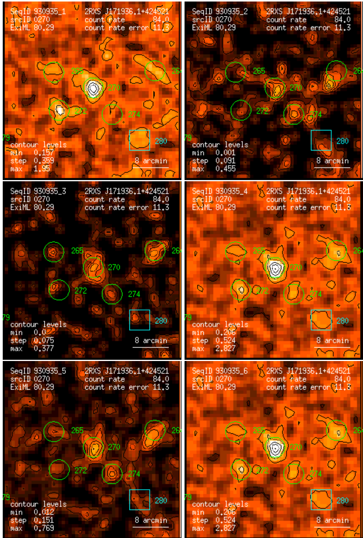
Figure 270: RASS 930935: detection 0270: band rate images, Gaussian filter: (1) PSPC channels 11 – 41, (2) 52 – 90, (3) 91 – 201, (4) 11 – 235, (5) 52 – 201, (6) 11 – 201. Broad band rates in counts/ks. Band rate contour levels in counts/ks/arcmin 2 .
