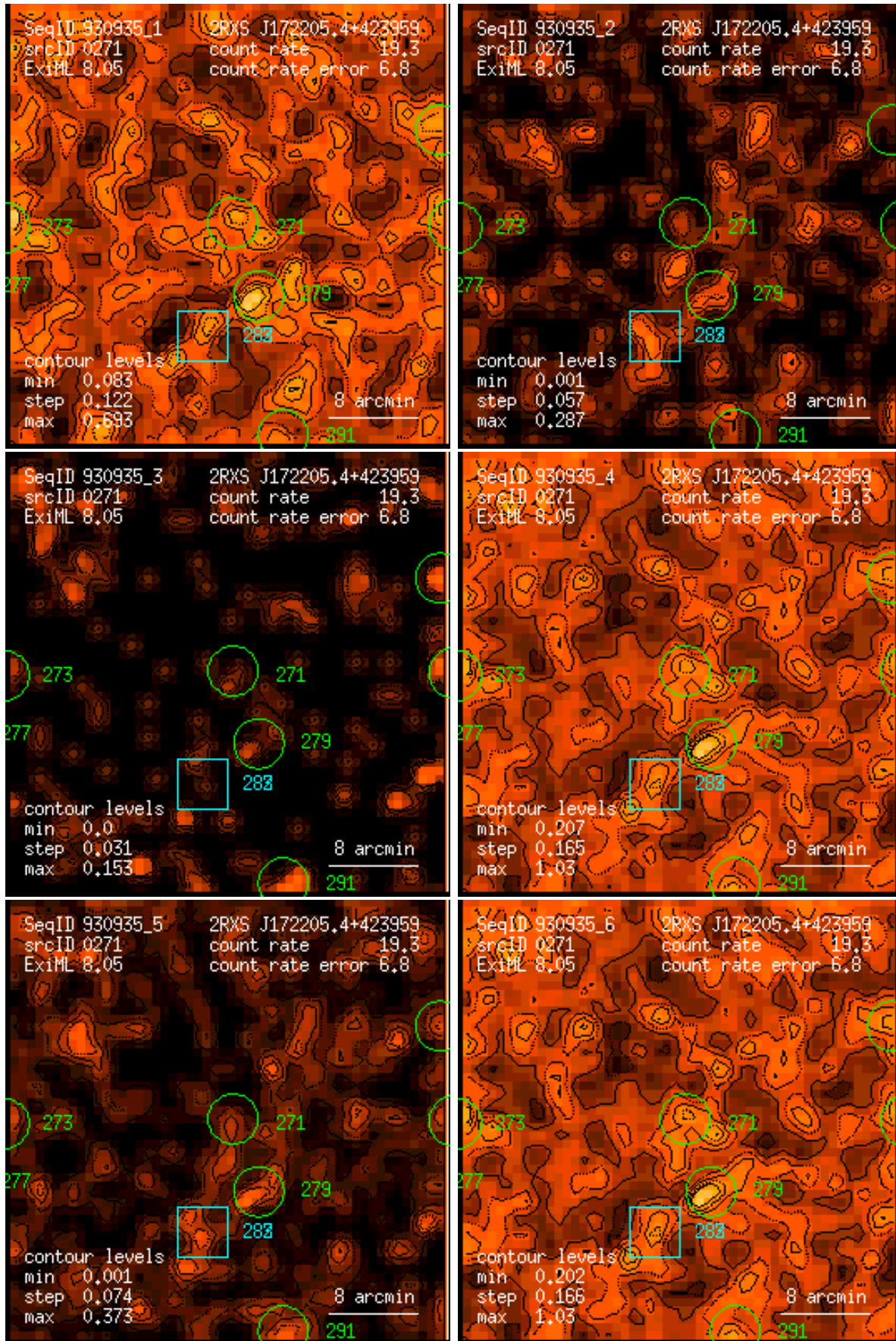
Figure 271: RASS 930935: detection 0271: band rate images, Gaussian filter: (1) PSPC channels 11 – 41, (2) 52 – 90, (3) 91 – 201, (4) 11 – 235, (5) 52 – 201, (6) 11 – 201. Broad band rates in counts/ks. Band rate contour levels in counts/ks/arcmin 2 .
