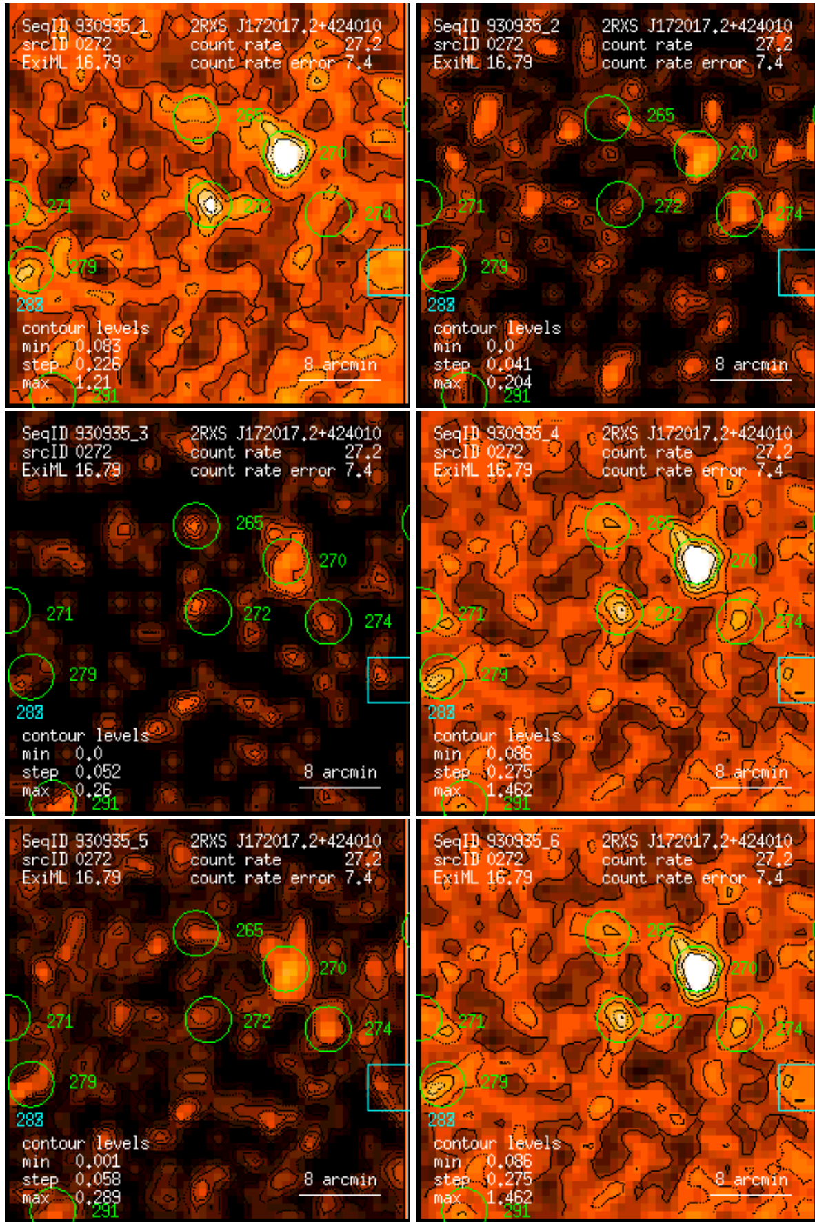
Figure 272: RASS 930935: detection 0272: band rate images, Gaussian filter: (1) PSPC channels 11 – 41, (2) 52 – 90, (3) 91 – 201, (4) 11 – 235, (5) 52 – 201, (6) 11 – 201. Broad band rates in counts/ks. Band rate contour levels in counts/ks/arcmin 2 .
