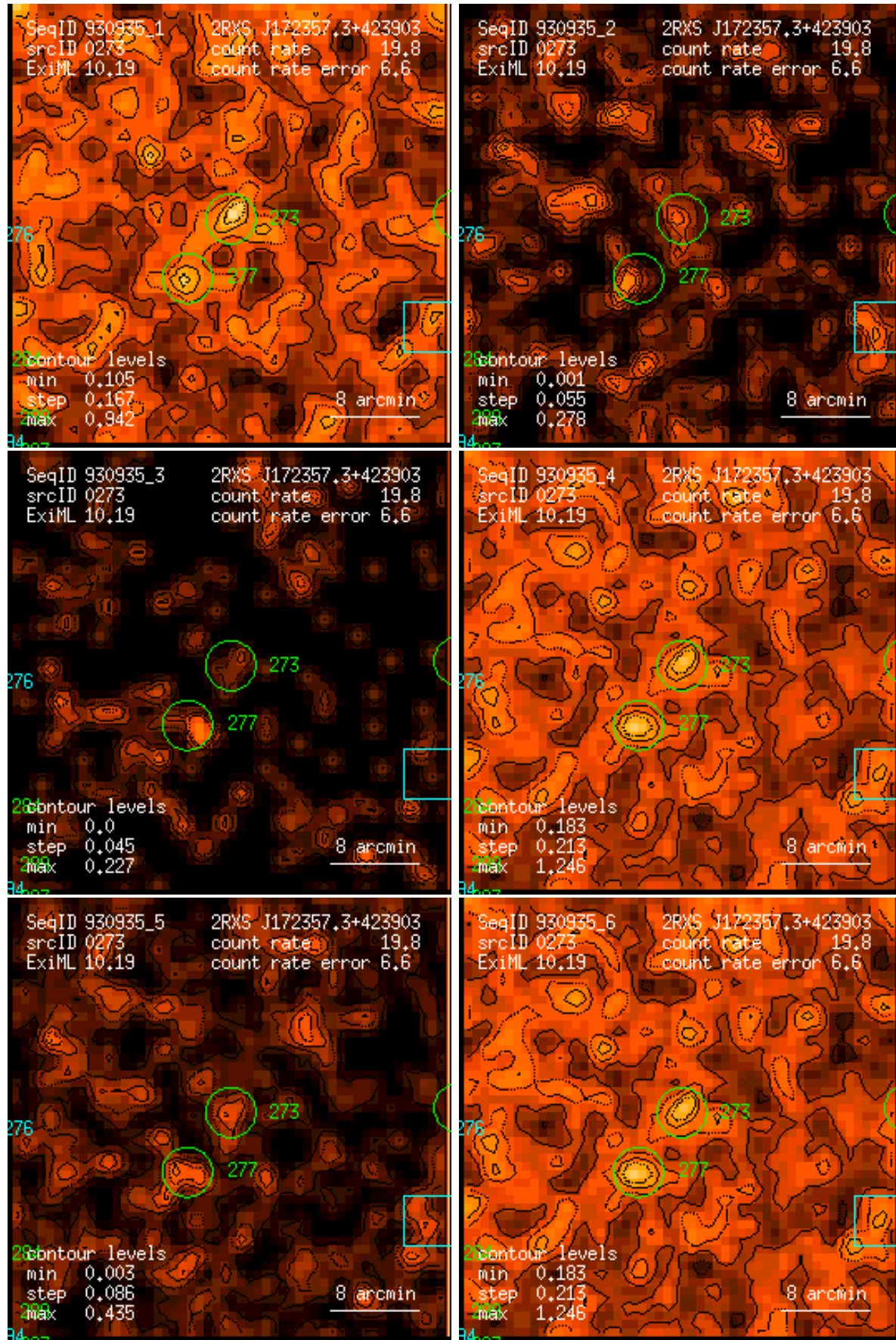
Figure 273: RASS 930935: detection 0273: band rate images, Gaussian filter: (1) PSPC channels 11 – 41, (2) 52 – 90, (3) 91 – 201, (4) 11 – 235, (5) 52 – 201, (6) 11 – 201. Broad band rates in counts/ks. Band rate contour levels in counts/ks/arcmin 2 .
