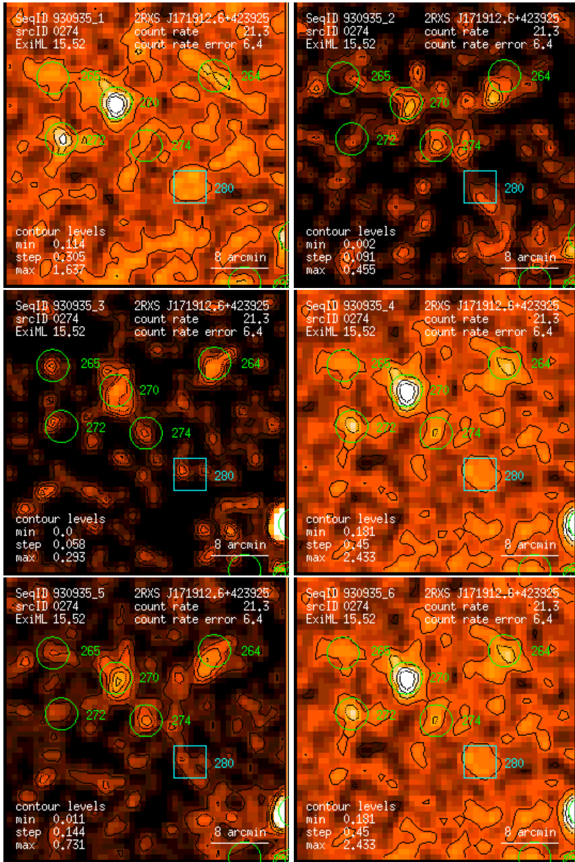
Figure 274: RASS 930935: detection 0274: band rate images, Gaussian filter: (1) PSPC channels 11 – 41, (2) 52 – 90, (3) 91 – 201, (4) 11 – 235, (5) 52 – 201, (6) 11 – 201. Broad band rates in counts/ks. Band rate contour levels in counts/ks/arcmin 2 .
