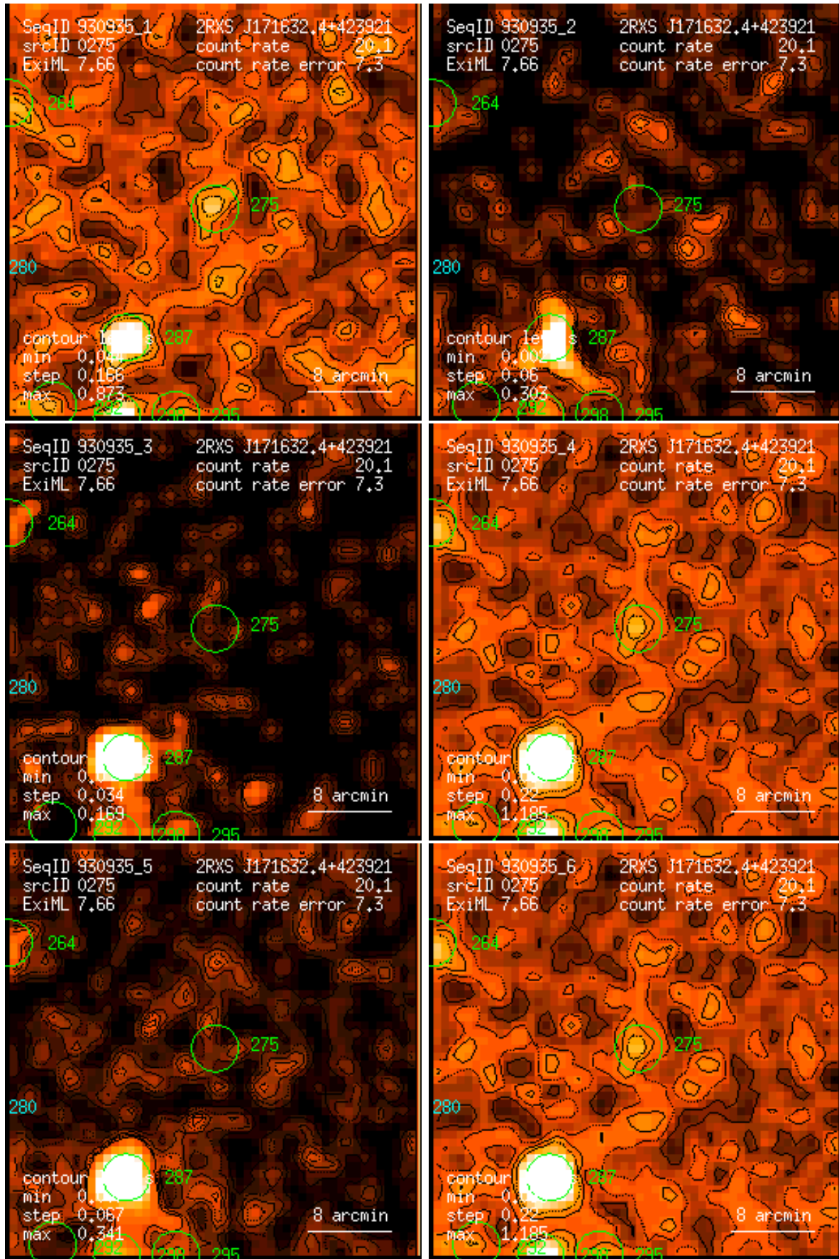
Figure 275: RASS 930935: detection 0275: band rate images, Gaussian filter: (1) PSPC channels 11 – 41, (2) 52 – 90, (3) 91 – 201, (4) 11 – 235, (5) 52 – 201, (6) 11 – 201. Broad band rates in counts/ks. Band rate contour levels in counts/ks/arcmin 2 .
