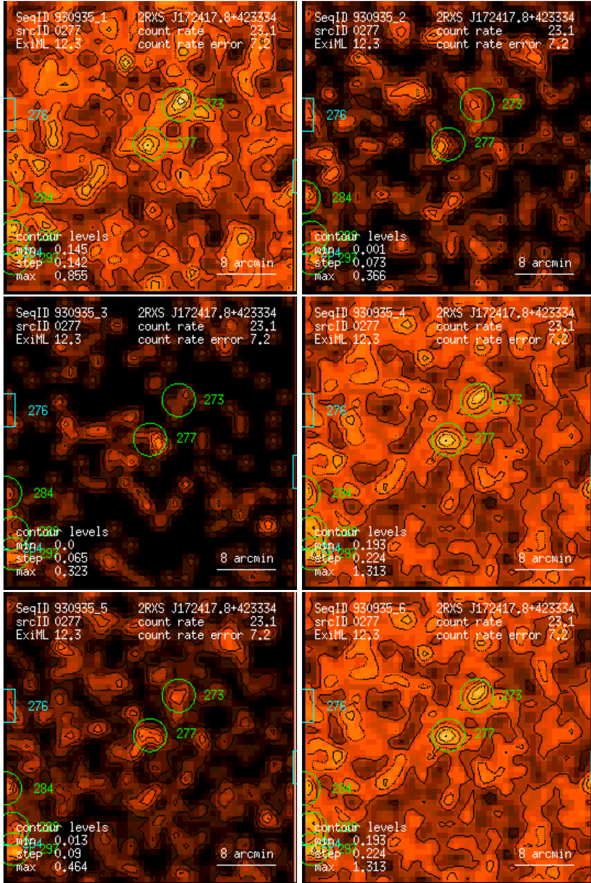
Figure 277: RASS 930935: detection 0277: band rate images, Gaussian filter: (1) PSPC channels 11 – 41, (2) 52 – 90, (3) 91 – 201, (4) 11 – 235, (5) 52 – 201, (6) 11 – 201. Broad band rates in counts/ks. Band rate contour levels in counts/ks/arcmin 2 .
