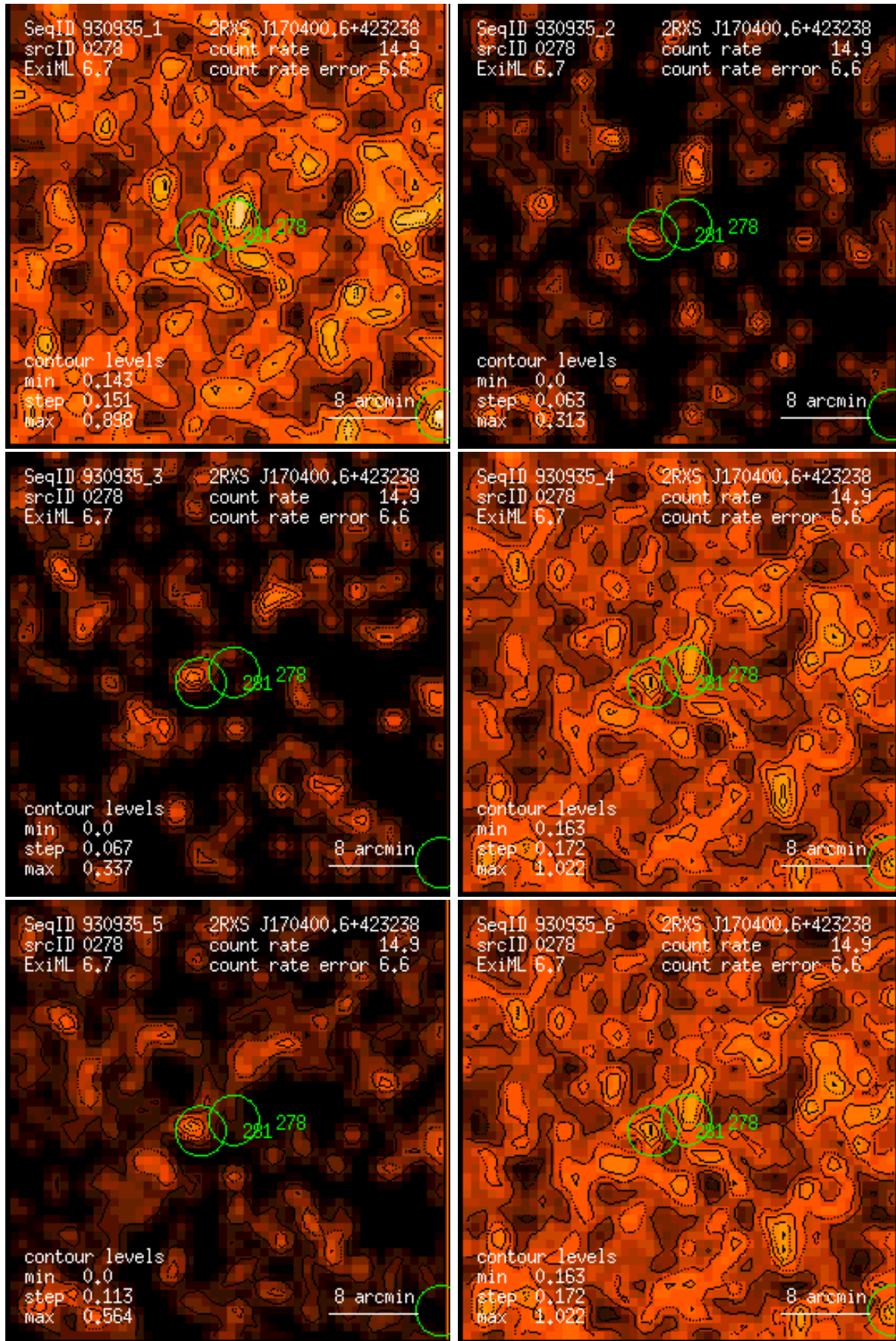
Figure 278: RASS 930935: detection 0278: band rate images, Gaussian filter: (1) PSPC channels 11 – 41, (2) 52 – 90, (3) 91 – 201, (4) 11 – 235, (5) 52 – 201, (6) 11 – 201. Broad band rates in counts/ks. Band rate contour levels in counts/ks/arcmin 2 .
