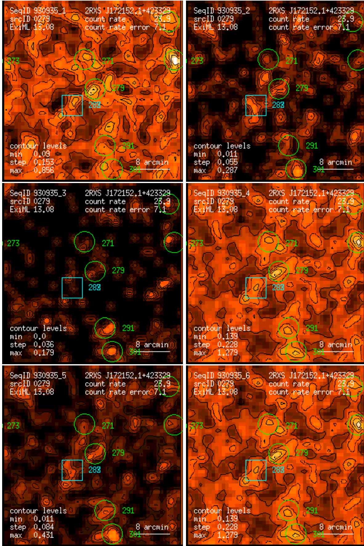
Figure 279: RASS 930935: detection 0279: band rate images, Gaussian filter: (1) PSPC channels 11 – 41, (2) 52 – 90, (3) 91 – 201, (4) 11 – 235, (5) 52 – 201, (6) 11 – 201. Broad band rates in counts/ks. Band rate contour levels in counts/ks/arcmin 2 .
