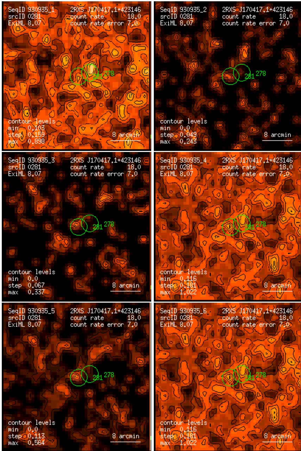
Figure 281: RASS 930935: detection 0281: band rate images, Gaussian filter: (1) PSPC channels 11 – 41, (2) 52 – 90, (3) 91 – 201, (4) 11 – 235, (5) 52 – 201, (6) 11 – 201. Broad band rates in counts/ks. Band rate contour levels in counts/ks/arcmin 2 .
