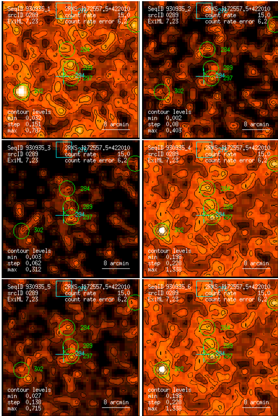
Figure 289: RASS 930935: detection 0289: band rate images, Gaussian filter: (1) PSPC channels 11 – 41, (2) 52 – 90, (3) 91 – 201, (4) 11 – 235, (5) 52 – 201, (6) 11 – 201. Broad band rates in counts/ks. Band rate contour levels in counts/ks/arcmin 2 .
