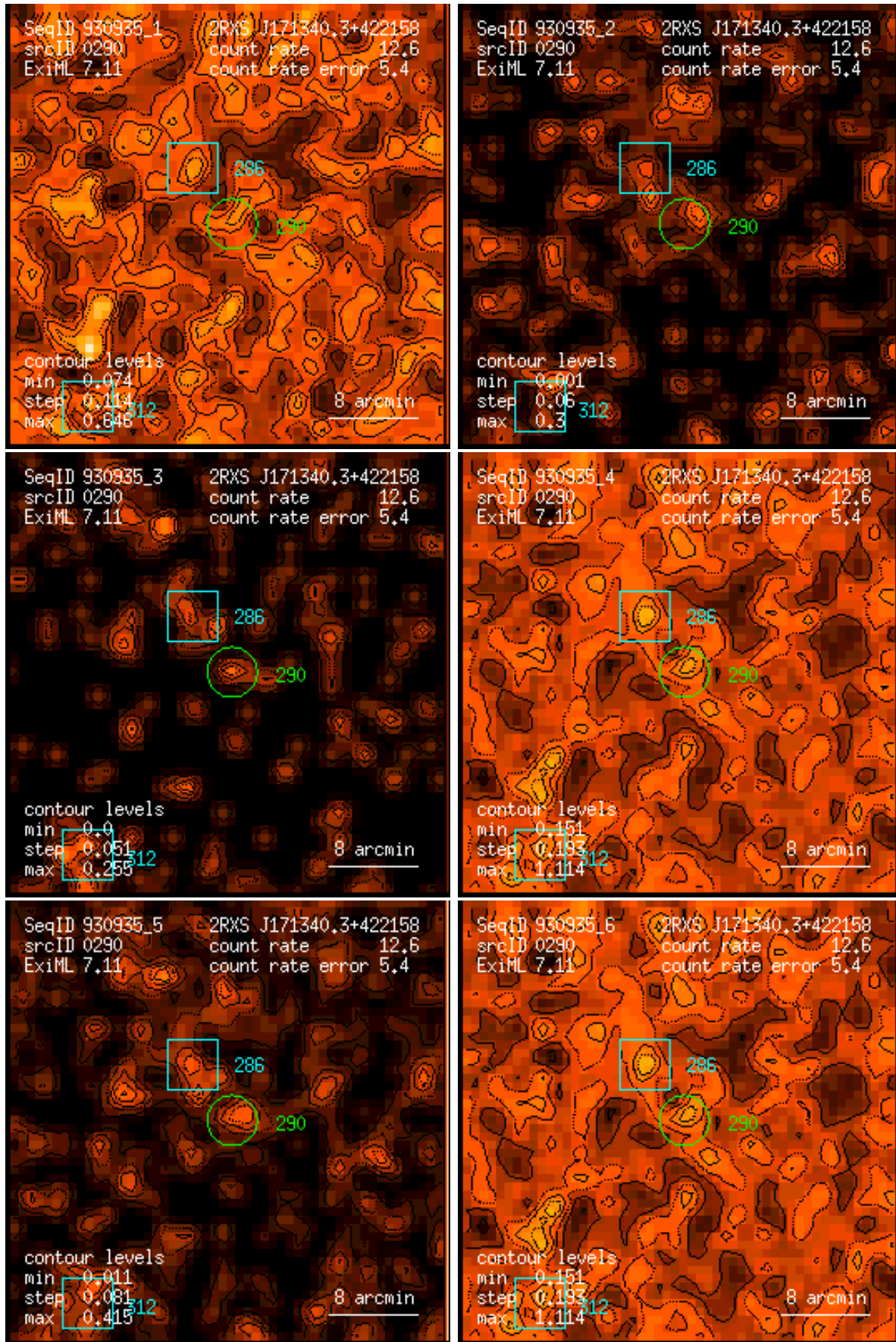
Figure 290: RASS 930935: detection 0290: band rate images, Gaussian filter: (1) PSPC channels 11 – 41, (2) 52 – 90, (3) 91 – 201, (4) 11 – 235, (5) 52 – 201, (6) 11 – 201. Broad band rates in counts/ks. Band rate contour levels in counts/ks/arcmin 2 .
