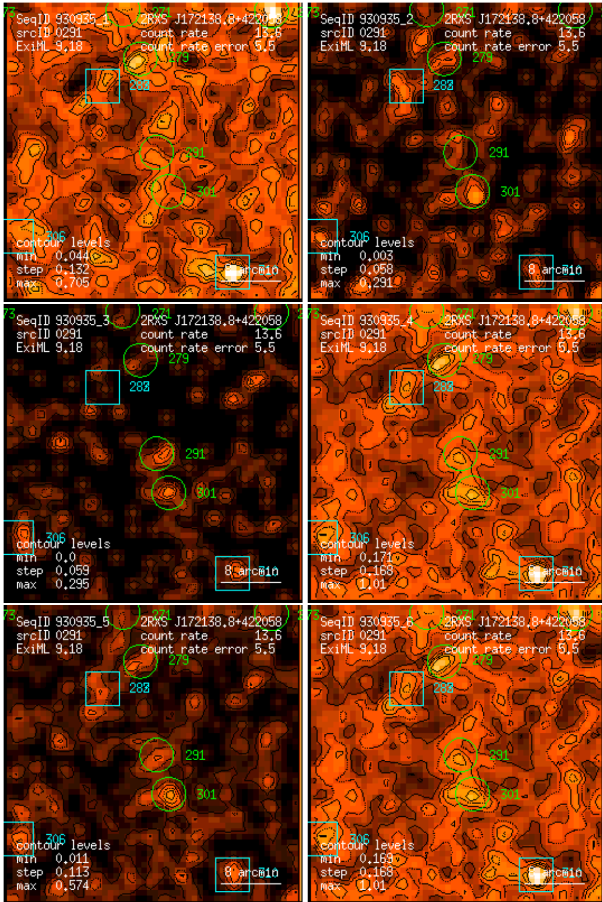
Figure 291: RASS 930935: detection 0291: band rate images, Gaussian filter: (1) PSPC channels 11 – 41, (2) 52 – 90, (3) 91 – 201, (4) 11 – 235, (5) 52 – 201, (6) 11 – 201. Broad band rates in counts/ks. Band rate contour levels in counts/ks/arcmin 2 .
