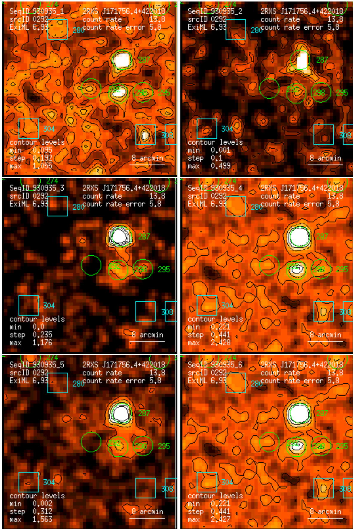
Figure 292: RASS 930935: detection 0292: band rate images, Gaussian filter: (1) PSPC channels 11 – 41, (2) 52 – 90, (3) 91 – 201, (4) 11 – 235, (5) 52 – 201, (6) 11 – 201. Broad band rates in counts/ks. Band rate contour levels in counts/ks/arcmin 2 .
