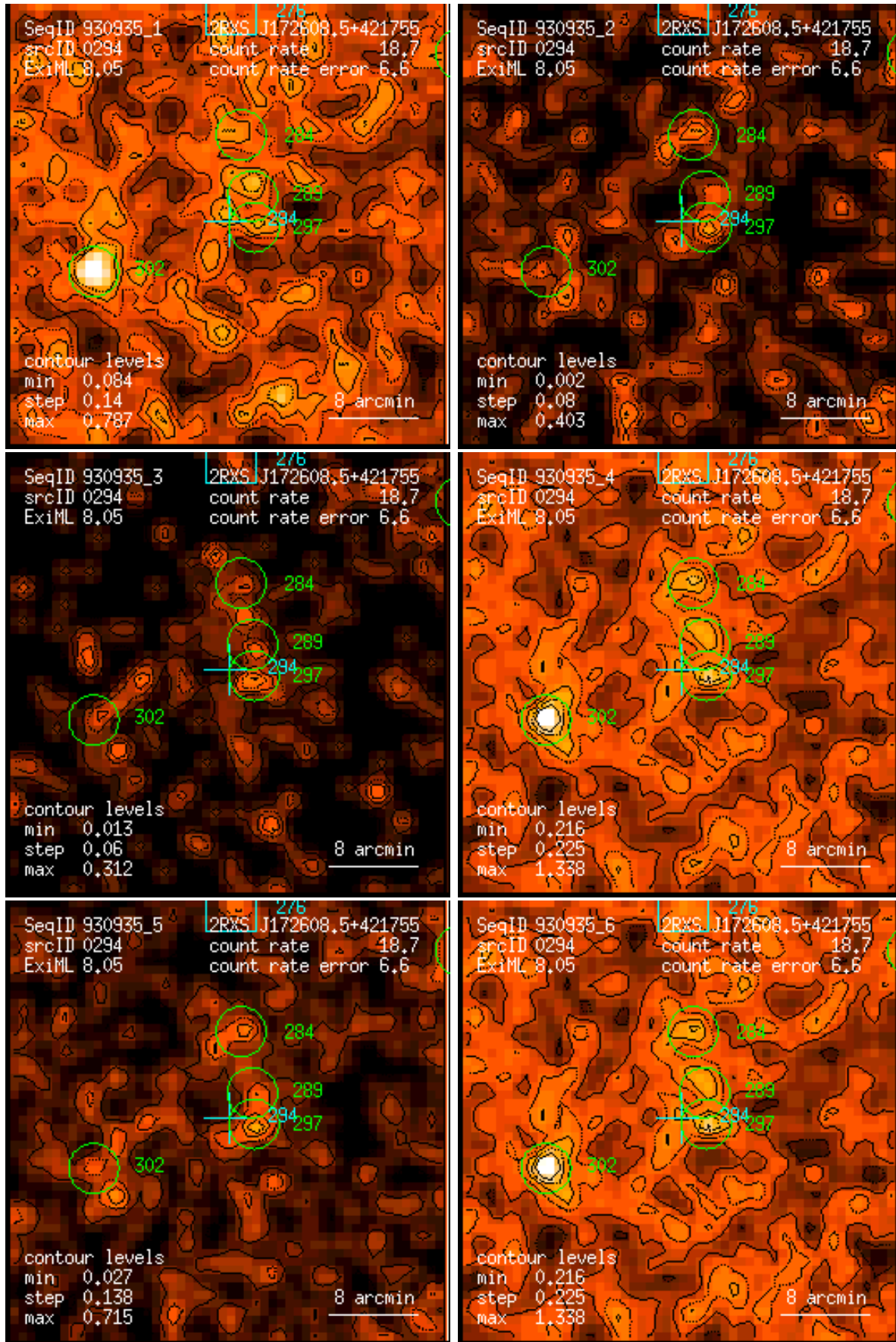
Figure 294: RASS 930935: detection 0294: band rate images, Gaussian filter: (1) PSPC channels 11 – 41, (2) 52 – 90, (3) 91 – 201, (4) 11 – 235, (5) 52 – 201, (6) 11 – 201. Broad band rates in counts/ks. Band rate contour levels in counts/ks/arcmin 2 .
