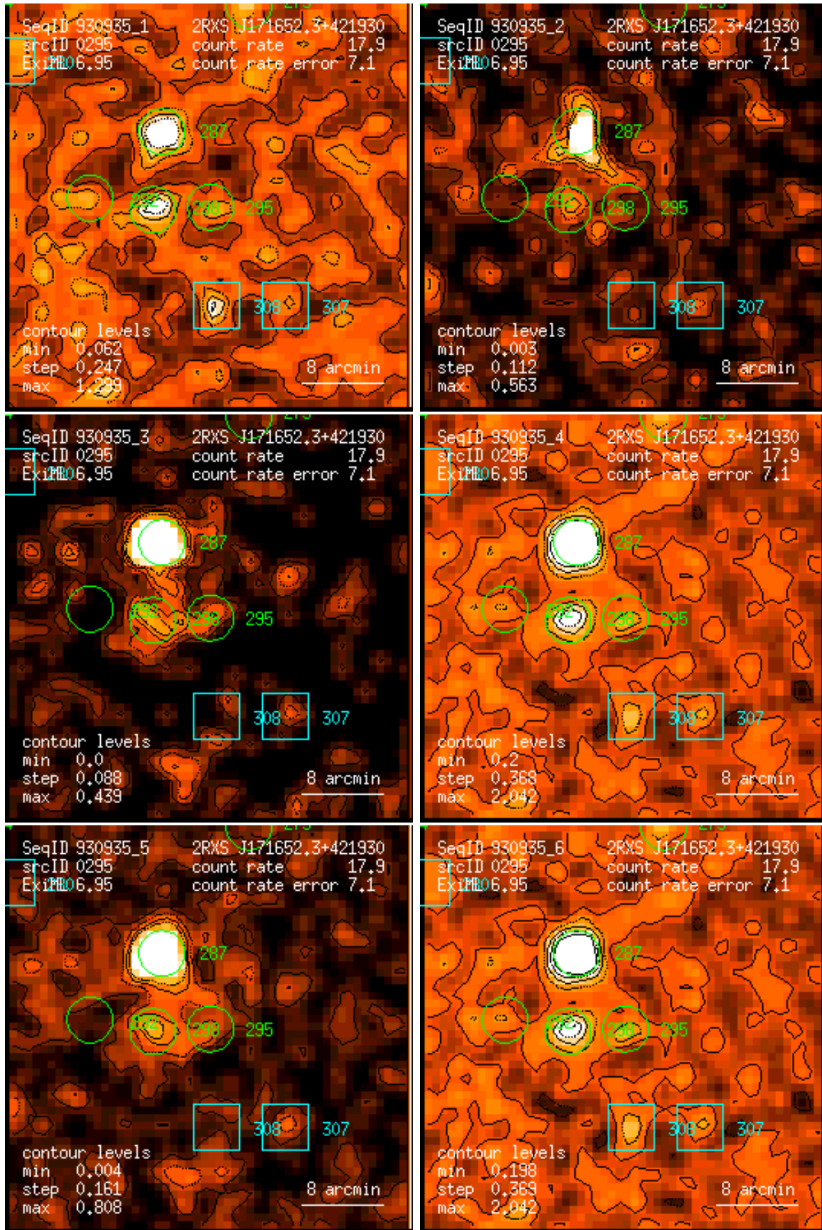
Figure 295: RASS 930935: detection 0295: band rate images, Gaussian filter: (1) PSPC channels 11 – 41, (2) 52 – 90, (3) 91 – 201, (4) 11 – 235, (5) 52 – 201, (6) 11 – 201. Broad band rates in counts/ks. Band rate contour levels in counts/ks/arcmin 2 .
