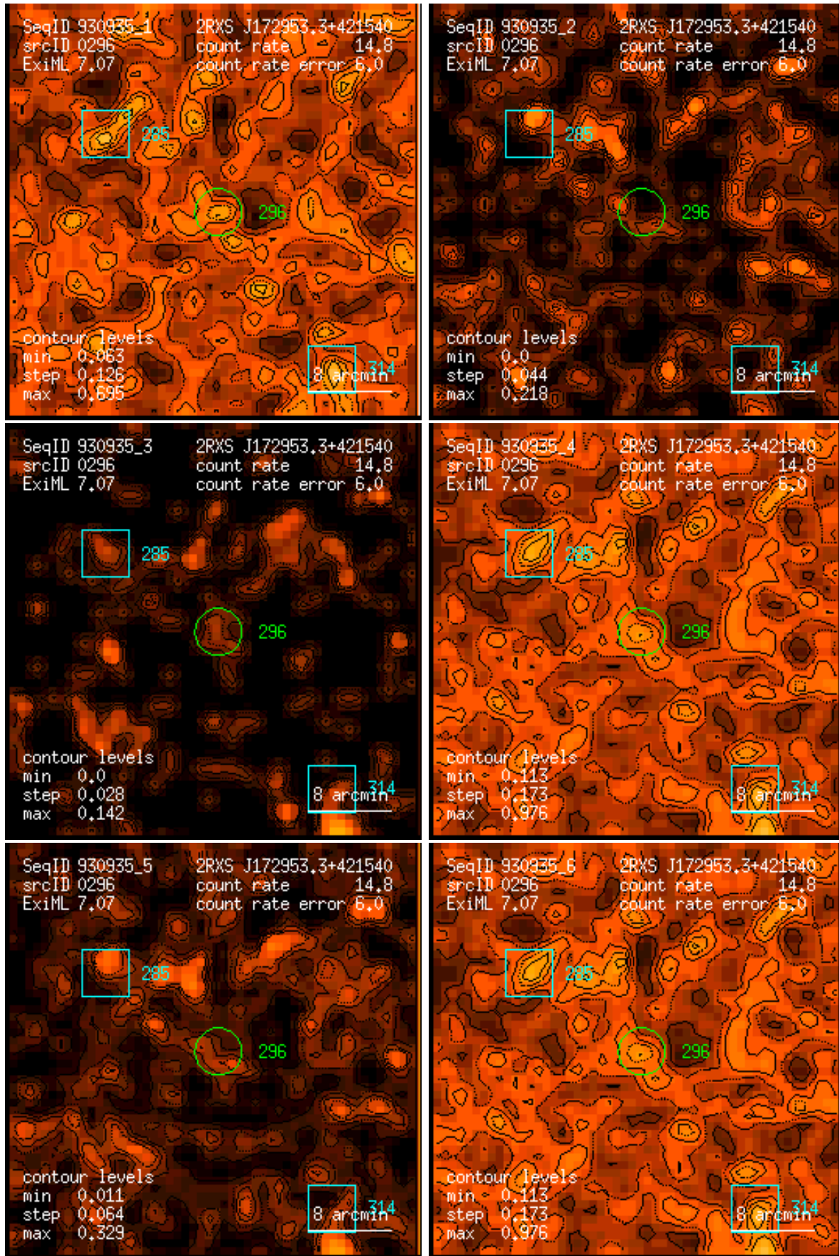
Figure 296: RASS 930935: detection 0296: band rate images, Gaussian filter: (1) PSPC channels 11 – 41, (2) 52 – 90, (3) 91 – 201, (4) 11 – 235, (5) 52 – 201, (6) 11 – 201. Broad band rates in counts/ks. Band rate contour levels in counts/ks/arcmin 2 .
