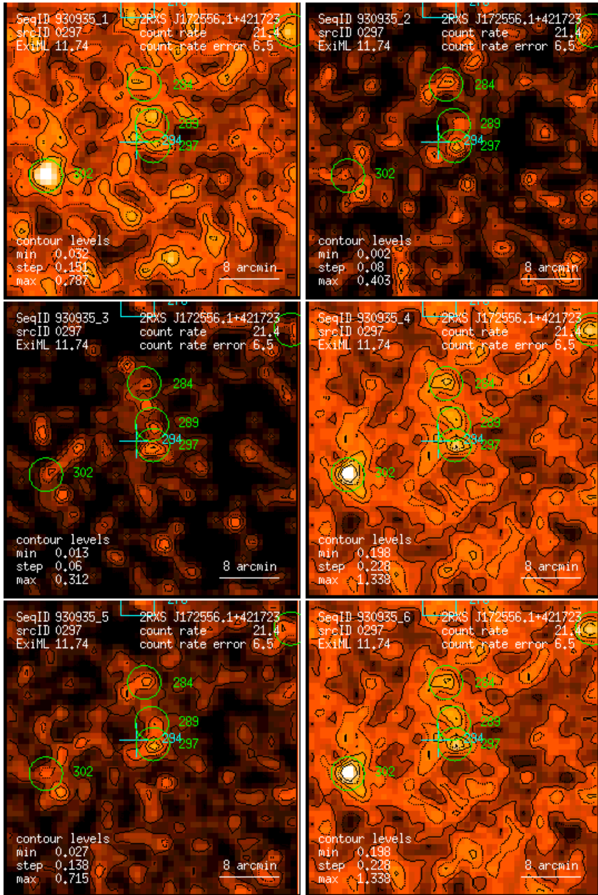
Figure 297: RASS 930935: detection 0297: band rate images, Gaussian filter: (1) PSPC channels 11 – 41, (2) 52 – 90, (3) 91 – 201, (4) 11 – 235, (5) 52 – 201, (6) 11 – 201. Broad band rates in counts/ks. Band rate contour levels in counts/ks/arcmin 2 .
