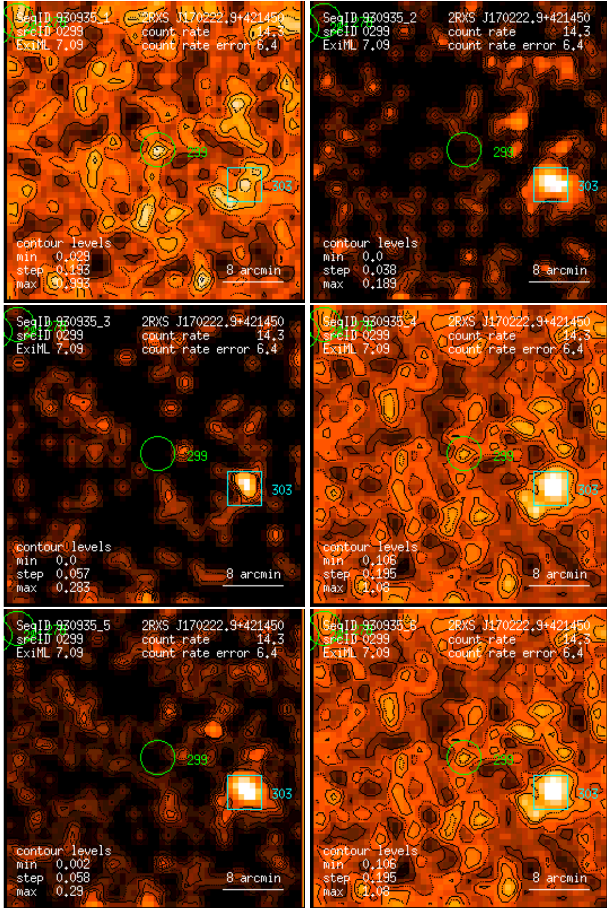
Figure 299: RASS 930935: detection 0299: band rate images, Gaussian filter: (1) PSPC channels 11 – 41, (2) 52 – 90, (3) 91 – 201, (4) 11 – 235, (5) 52 – 201, (6) 11 – 201. Broad band rates in counts/ks. Band rate contour levels in counts/ks/arcmin 2 .
