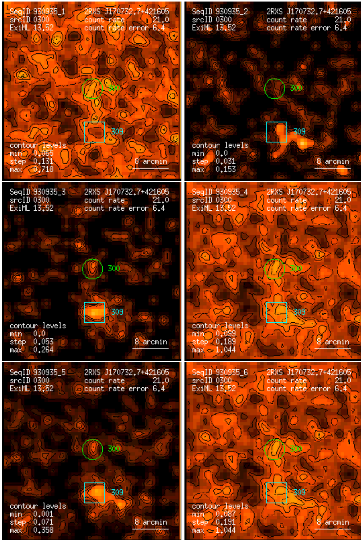
Figure 300: RASS 930935: detection 0300: band rate images, Gaussian filter: (1) PSPC channels 11 – 41, (2) 52 – 90, (3) 91 – 201, (4) 11 – 235, (5) 52 – 201, (6) 11 – 201. Broad band rates in counts/ks. Band rate contour levels in counts/ks/arcmin 2 .
