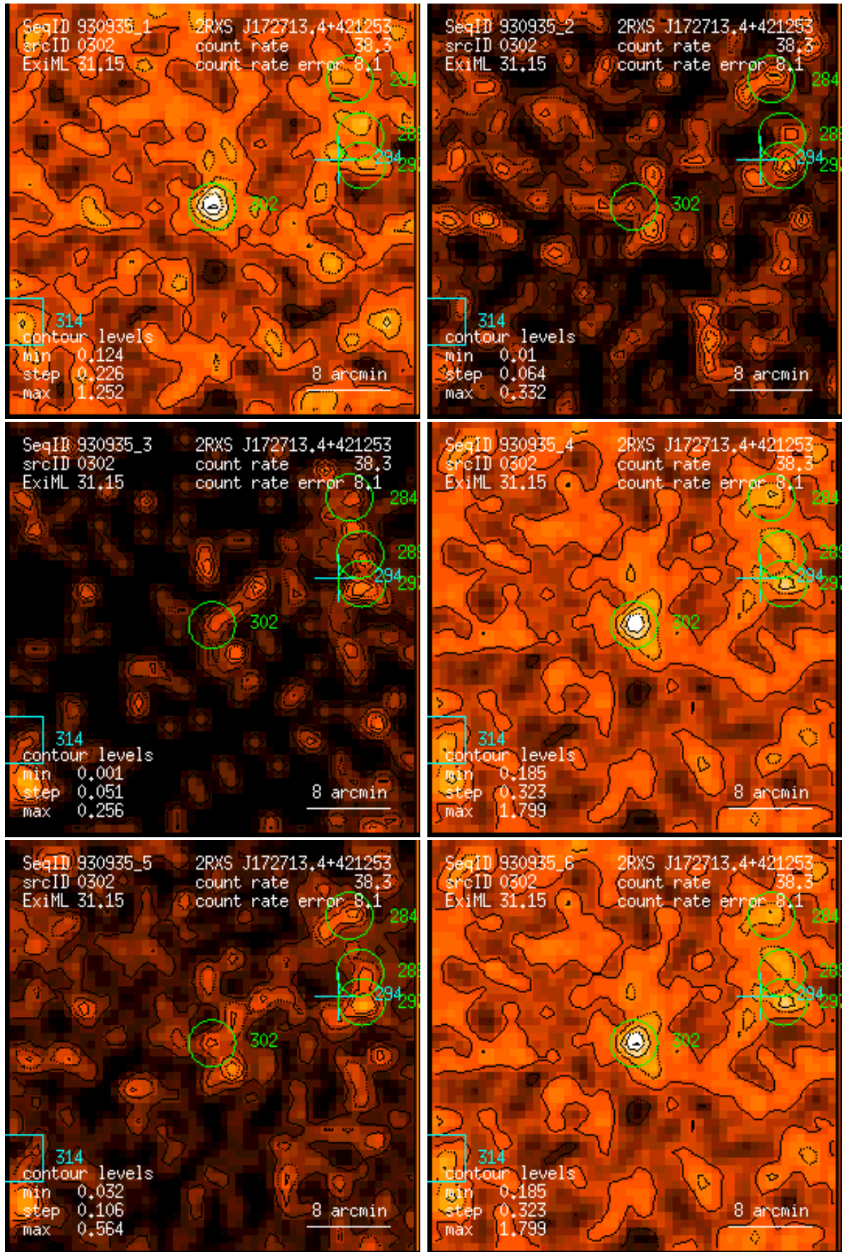
Figure 302: RASS 930935: detection 0302: band rate images, Gaussian filter: (1) PSPC channels 11 – 41, (2) 52 – 90, (3) 91 – 201, (4) 11 – 235, (5) 52 – 201, (6) 11 – 201. Broad band rates in counts/ks. Band rate contour levels in counts/ks/arcmin 2 .
