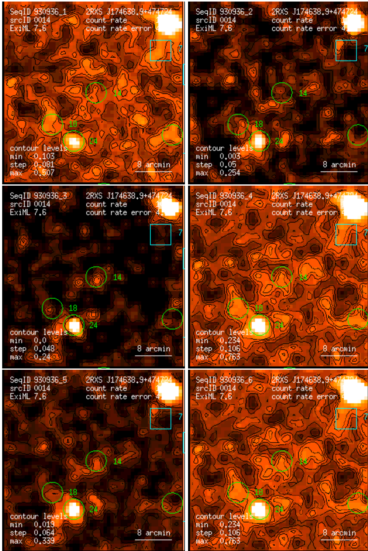
Figure 14: RASS 930936: detection 0014: band rate images, Gaussian filter: (1) PSPC channels 11 – 41, (2) 52 – 90, (3) 91 – 201, (4) 11 – 235, (5) 52 – 201, (6) 11 – 201. Broad band rates in counts/ks. Band rate contour levels in counts/ks/arcmin 2 .
