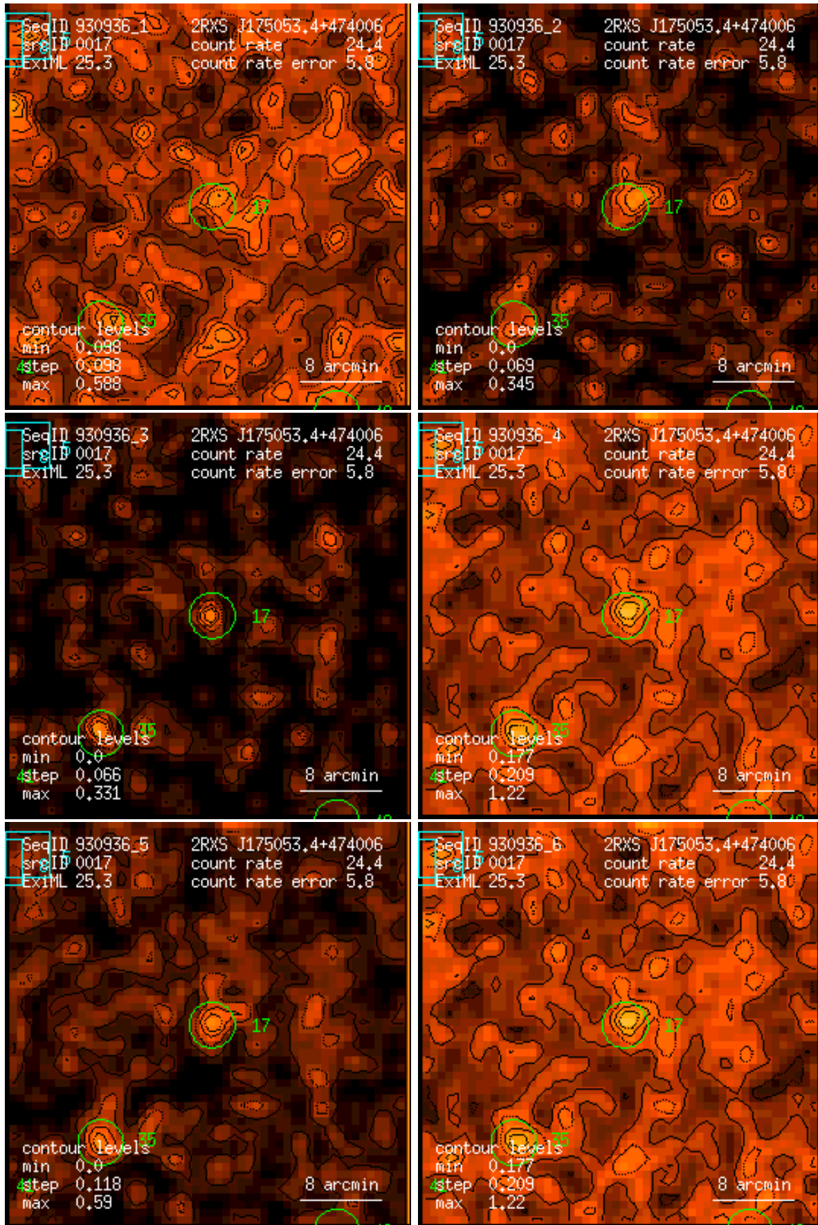
Figure 17: RASS 930936: detection 0017: band rate images, Gaussian filter: (1) PSPC channels 11 – 41, (2) 52 – 90, (3) 91 – 201, (4) 11 – 235, (5) 52 – 201, (6) 11 – 201. Broad band rates in counts/ks. Band rate contour levels in counts/ks/arcmin 2 .
