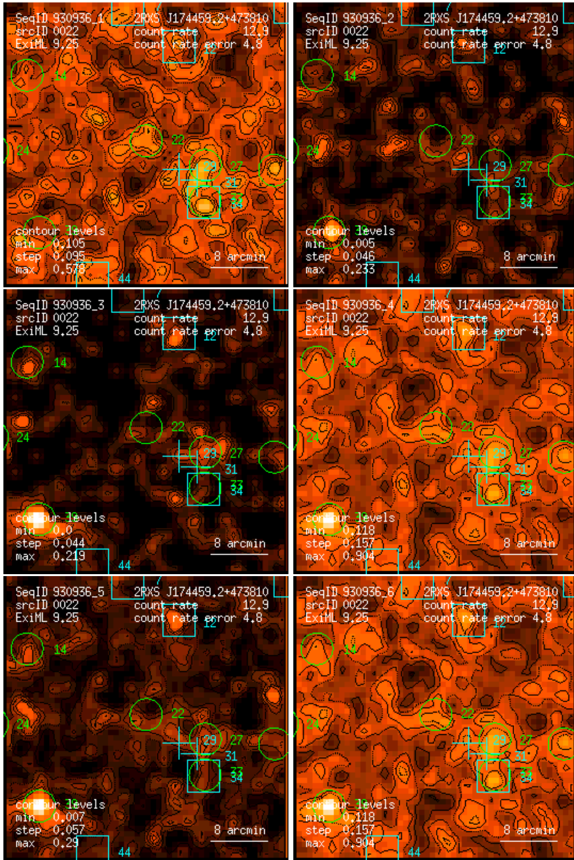
Figure 22: RASS 930936: detection 0022: band rate images, Gaussian filter: (1) PSPC channels 11 – 41, (2) 52 – 90, (3) 91 – 201, (4) 11 – 235, (5) 52 – 201, (6) 11 – 201. Broad band rates in counts/ks. Band rate contour levels in counts/ks/arcmin 2 .
