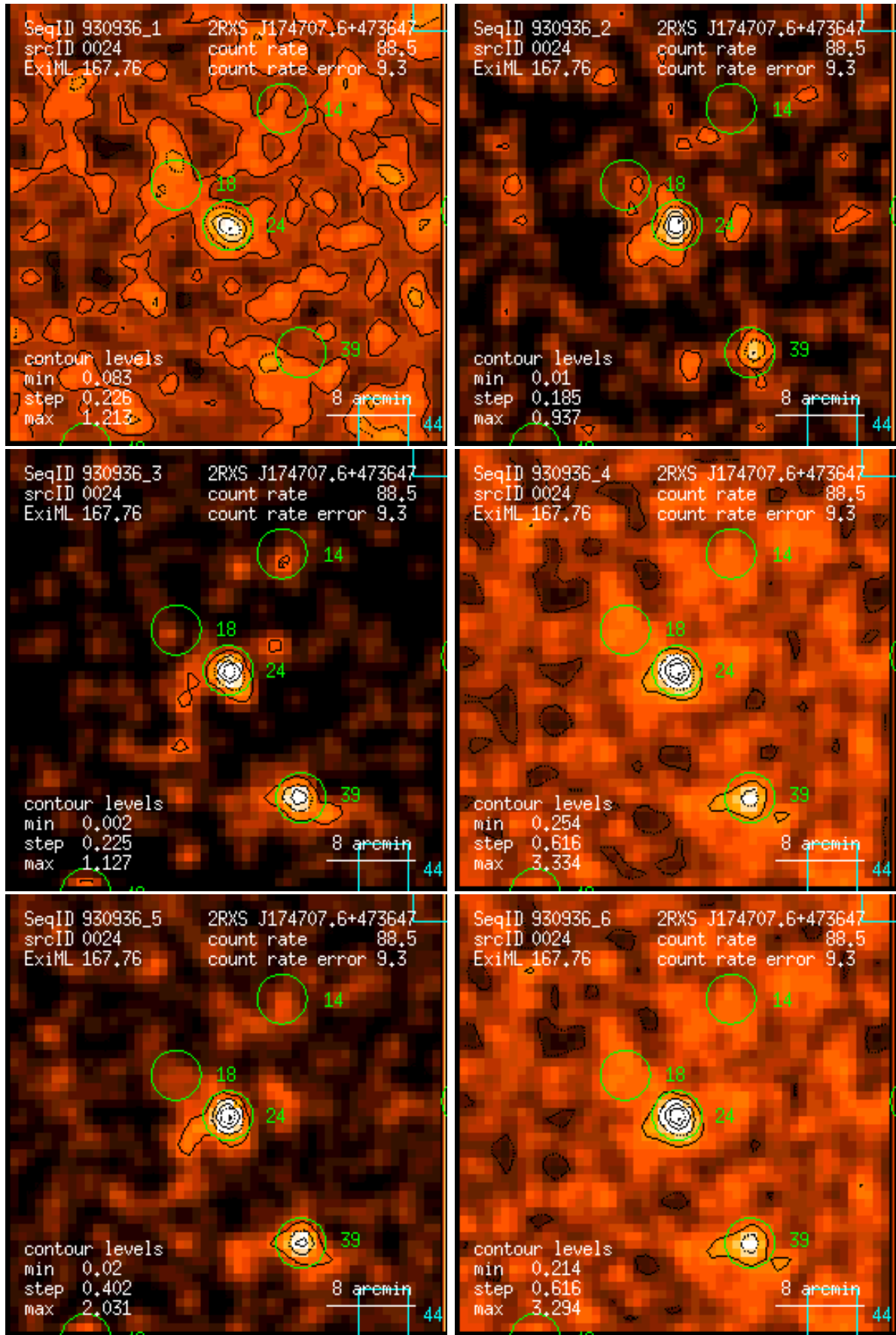
Figure 24: RASS 930936: detection 0024: band rate images, Gaussian filter: (1) PSPC channels 11 – 41, (2) 52 – 90, (3) 91 – 201, (4) 11 – 235, (5) 52 – 201, (6) 11 – 201. Broad band rates in counts/ks. Band rate contour levels in counts/ks/arcmin 2 .
