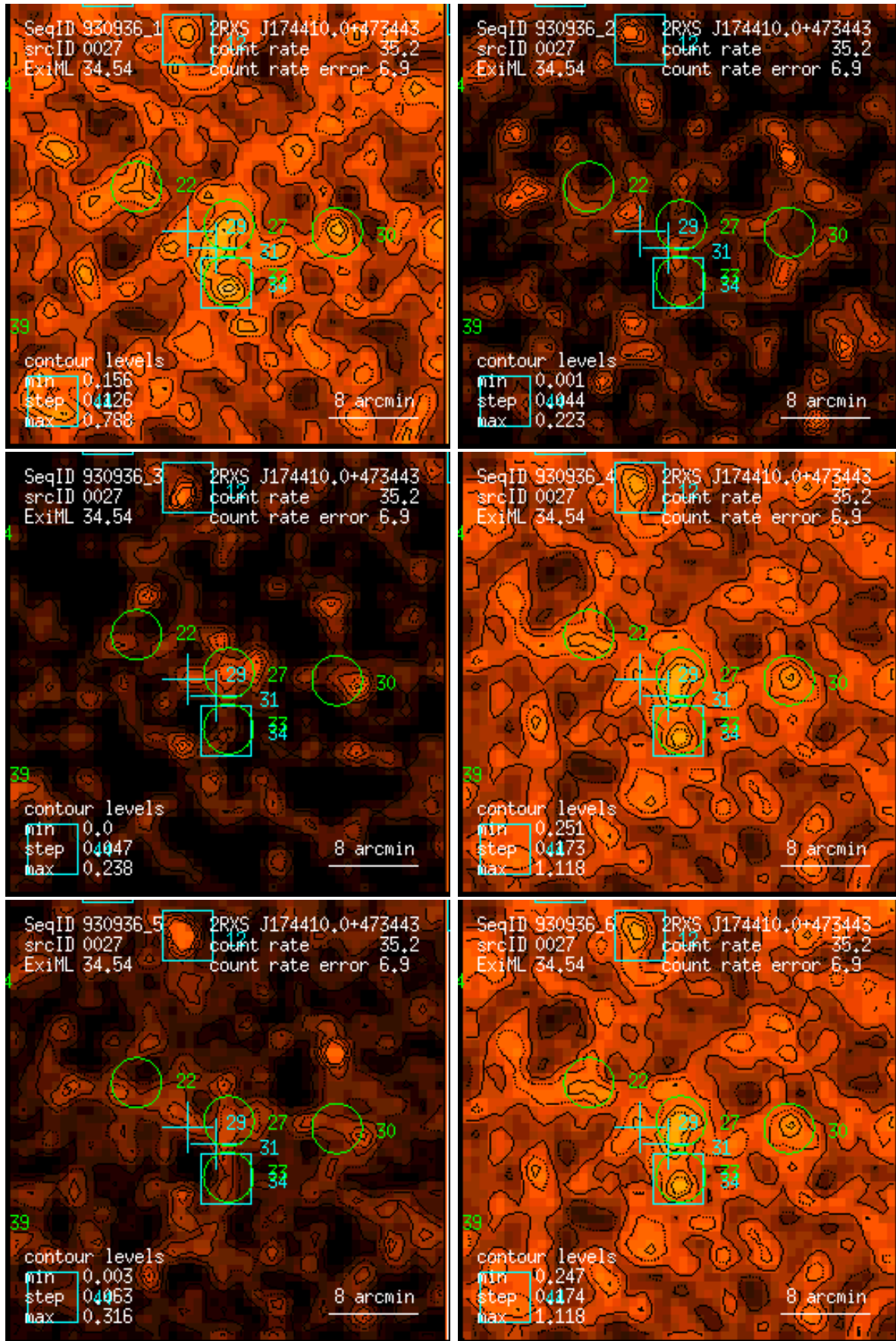
Figure 27: RASS 930936: detection 0027: band rate images, Gaussian filter: (1) PSPC channels 11 – 41, (2) 52 – 90, (3) 91 – 201, (4) 11 – 235, (5) 52 – 201, (6) 11 – 201. Broad band rates in counts/ks. Band rate contour levels in counts/ks/arcmin 2 .
