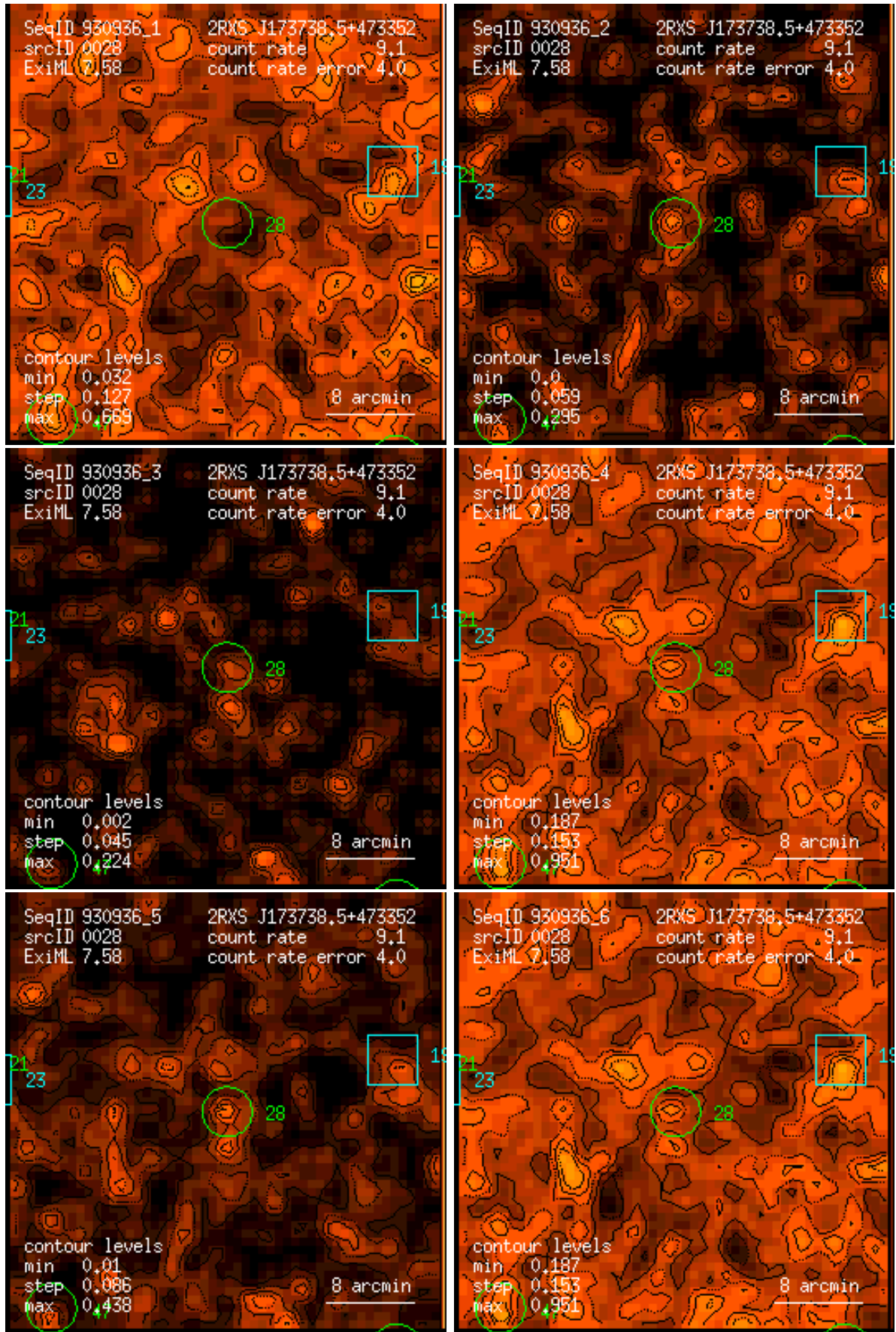
Figure 28: RASS 930936: detection 0028: band rate images, Gaussian filter: (1) PSPC channels 11 – 41, (2) 52 – 90, (3) 91 – 201, (4) 11 – 235, (5) 52 – 201, (6) 11 – 201. Broad band rates in counts/ks. Band rate contour levels in counts/ks/arcmin 2 .
