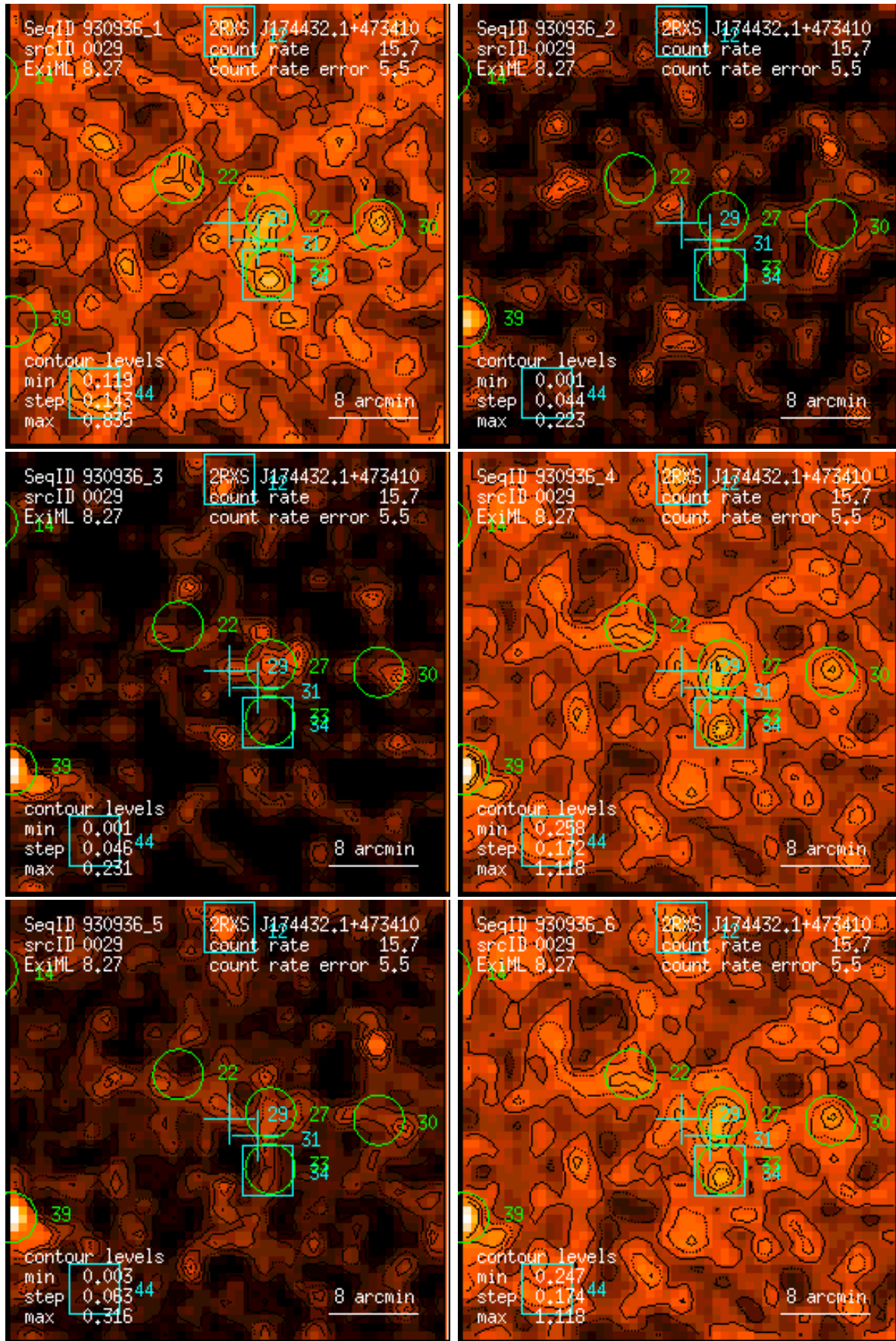
Figure 29: RASS 930936: detection 0029: band rate images, Gaussian filter: (1) PSPC channels 11 – 41, (2) 52 – 90, (3) 91 – 201, (4) 11 – 235, (5) 52 – 201, (6) 11 – 201. Broad band rates in counts/ks. Band rate contour levels in counts/ks/arcmin 2 .
