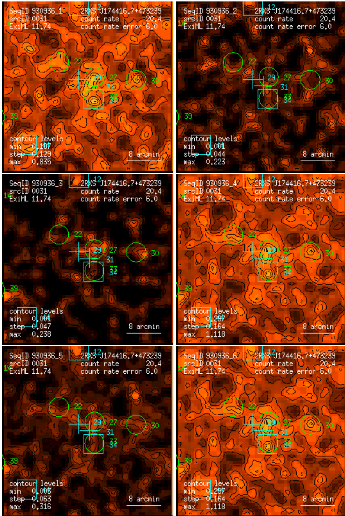
Figure 31: RASS 930936: detection 0031: band rate images, Gaussian filter: (1) PSPC channels 11 – 41, (2) 52 – 90, (3) 91 – 201, (4) 11 – 235, (5) 52 – 201, (6) 11 – 201. Broad band rates in counts/ks. Band rate contour levels in counts/ks/arcmin 2 .
