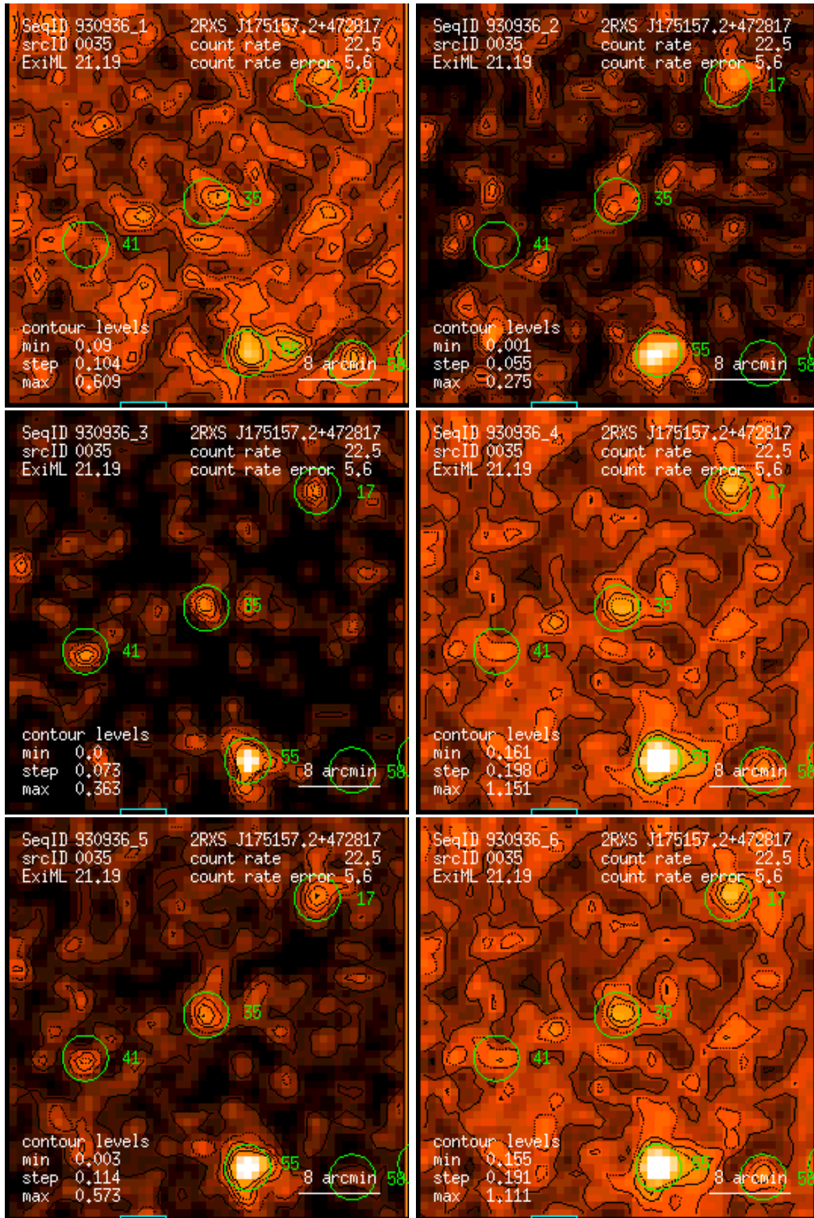
Figure 35: RASS 930936: detection 0035: band rate images, Gaussian filter: (1) PSPC channels 11 – 41, (2) 52 – 90, (3) 91 – 201, (4) 11 – 235, (5) 52 – 201, (6) 11 – 201. Broad band rates in counts/ks. Band rate contour levels in counts/ks/arcmin 2 .
