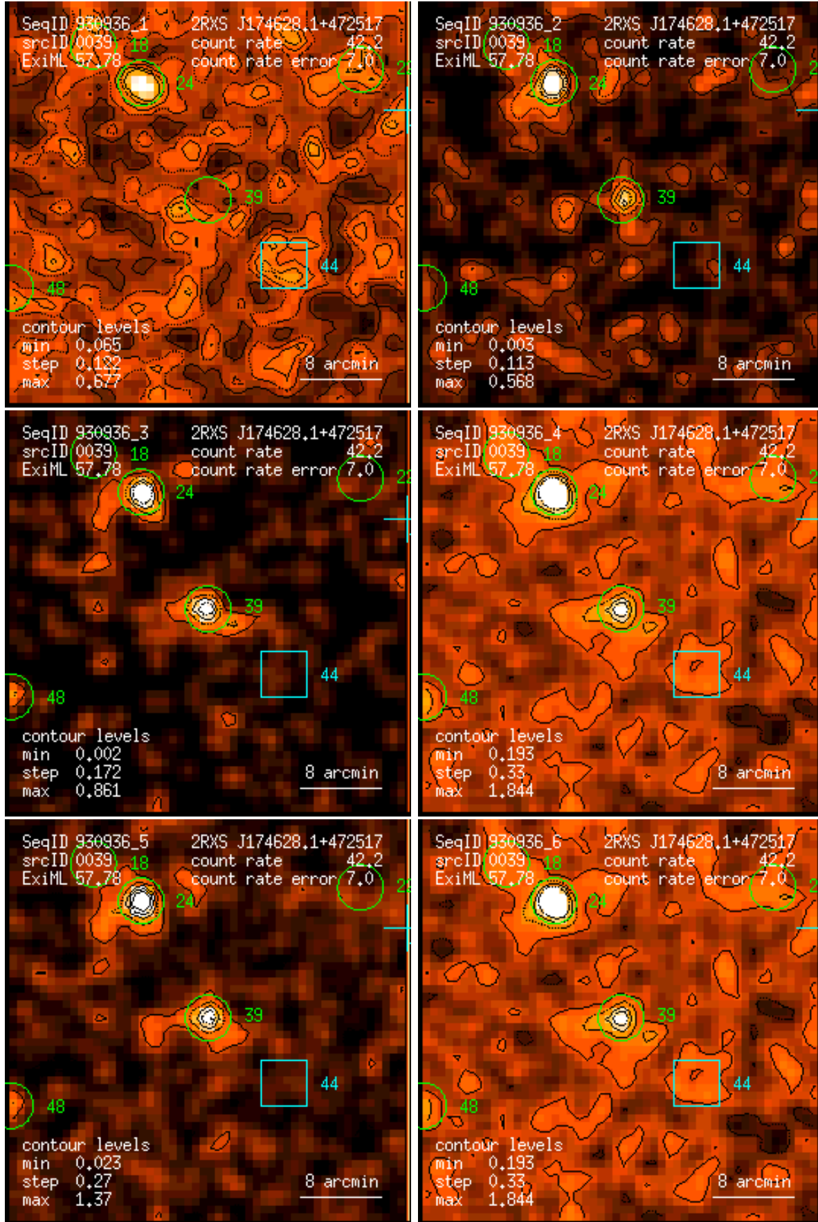
Figure 39: RASS 930936: detection 0039: band rate images, Gaussian filter: (1) PSPC channels 11 – 41, (2) 52 – 90, (3) 91 – 201, (4) 11 – 235, (5) 52 – 201, (6) 11 – 201. Broad band rates in counts/ks. Band rate contour levels in counts/ks/arcmin 2 .
