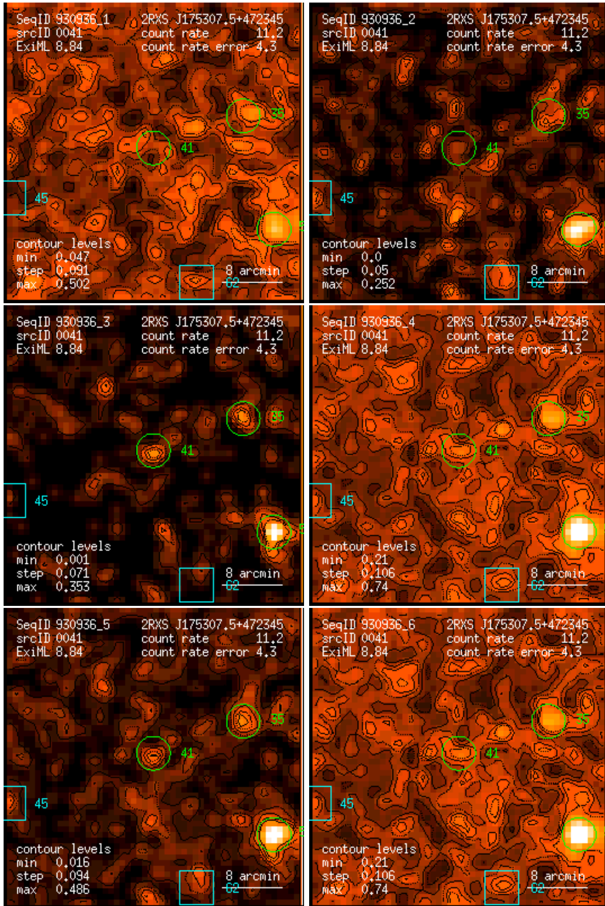
Figure 41: RASS 930936: detection 0041: band rate images, Gaussian filter: (1) PSPC channels 11 – 41, (2) 52 – 90, (3) 91 – 201, (4) 11 – 235, (5) 52 – 201, (6) 11 – 201. Broad band rates in counts/ks. Band rate contour levels in counts/ks/arcmin 2 .
